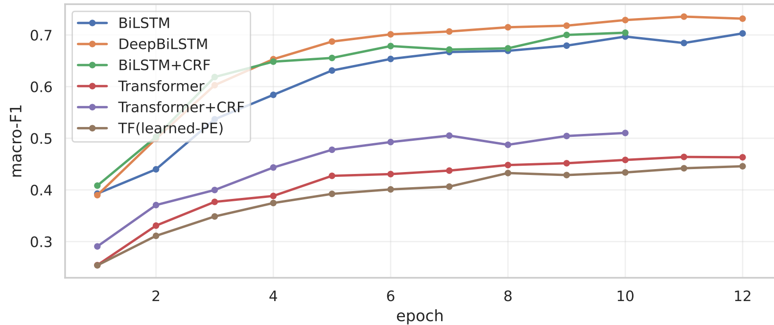
Validation macro-F1 across epochs
