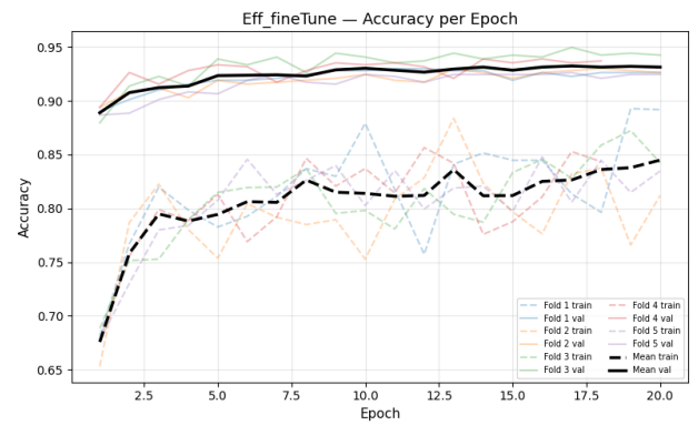
(f) Eff-B3 Fine-Tune — Accuracy
