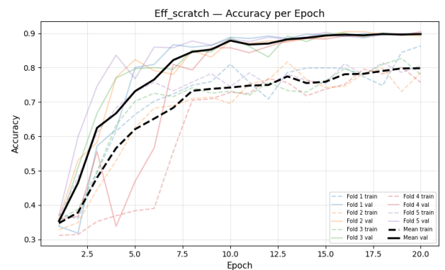
(h) Eff-B3 Scratch — Accuracy
