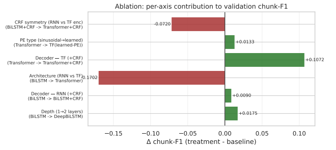
Figure 2: Ablation \Delta ChunkF1 for six single-axis comparisons.
