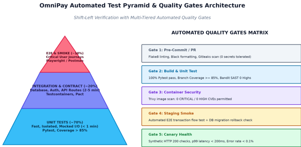
Figure 4: Automated Test Pyramid Distribution and Quality Gates Matrix.
