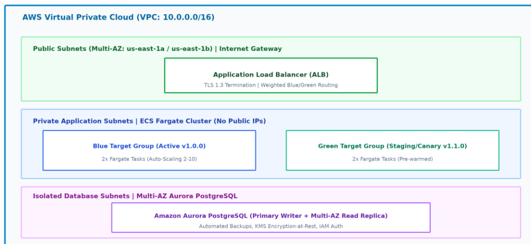
Figure 5: OmniPay AWS Cloud Infrastructure Topology Provisioned via Terraform.
