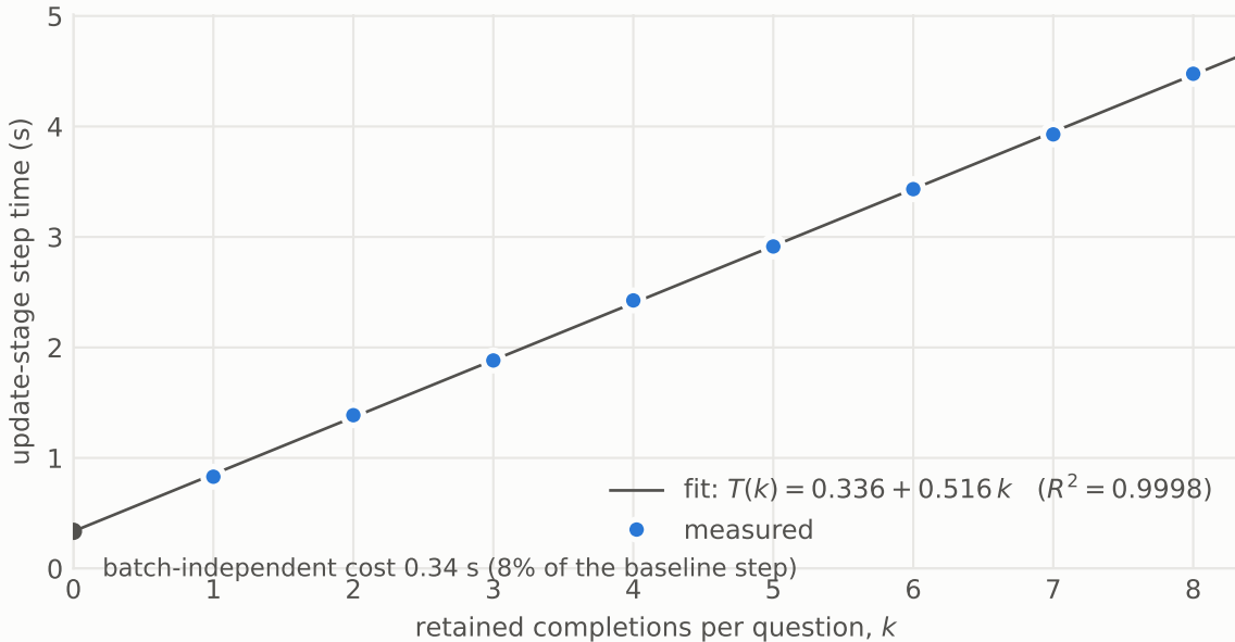
Update stage is linear in k — Qwen/Qwen3-0.6B, G = 8
