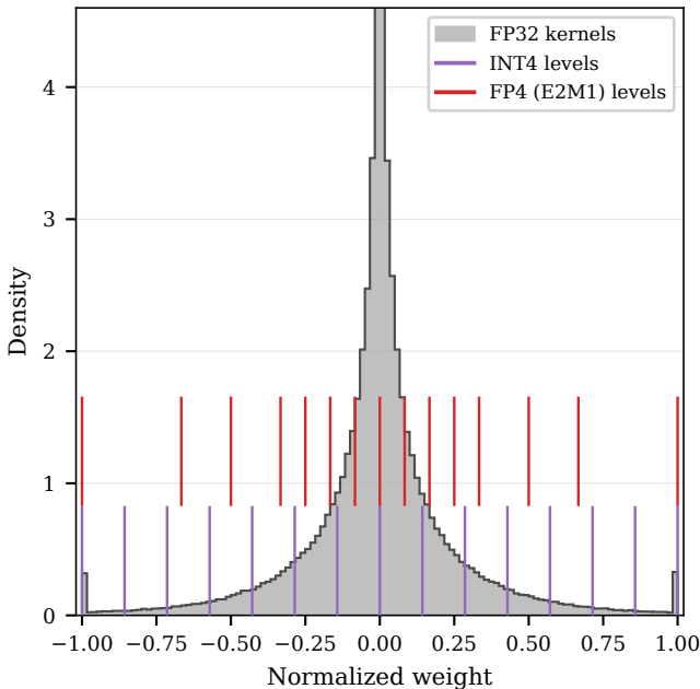
Weight mass concentrates at zero
