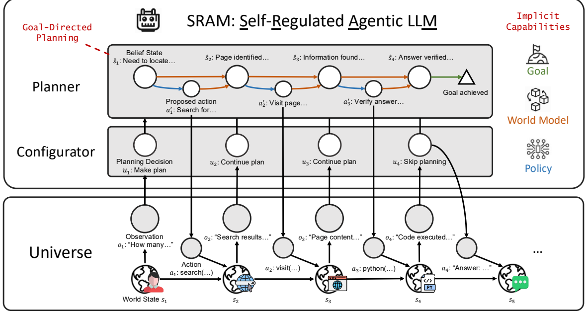
Figure 1: Illustration of the decision-making process of SRAM. The agentic LLM interacts with the universe over multiple time steps, receiving observations o_t and executing actions a_t . At each step, the configurator outputs decision u_t for whether to make a new plan, continue an existing plan, or skip planning entirely. When planning is invoked, the planner simulates a sequence of proposed actions a'_t and predicted belief states \hat{s}_{t+1} conditioned on the current state \hat{s}_t , implicitly performing goal-directed planning with world-model simulation (right labels). Both the configurator and the planner are realized in the same LLM, with their outputs distinguished by structured generation. The example depicts a web information-seeking task where the model first carefully plans a search-and-visit strategy, continues executing the plan at steps 2 and 3, and skips planning at step 4 to provide an answer to the user.
