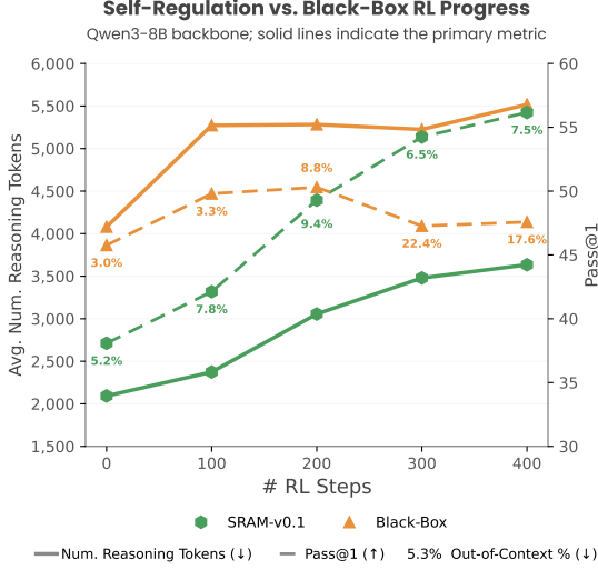
Figure 5: RL training progress over 400 steps from supervised self-regulation training (v0.1, green) vs. base model with black-box reasoning (orange). Solid lines show average reasoning tokens per trajectory (left axis, ↓ better); dashed lines show overall Pass@1 (right axis, ↑ better); percentages indicate out-of-context rate (↓ better) at each checkpoint. Without self-regulation structure, RL increases token consumption with diminishing accuracy returns, while self-regulated model achieves steadily improving accuracy with controlled token growth.
