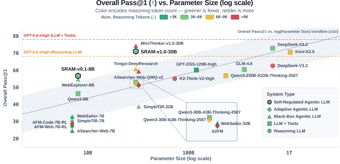
Figure 2: Overall Pass Rate vs. Parameter Size across all evaluated systems. Marker shape denotes system type; color encodes average reasoning token count per trajectory (greener = fewer, redder = more). The trendline and shaded band show the linear fit ( \pm 1\sigma ) of Overall Pass@1 against Log Parameter Size. Dashed orange/red line mark GPT-5.4-xhigh performance as Reasoning LLM and LLM + Tools for reference. Both SRAM models sit above the scaling trend, achieving accuracy competitive with substantially larger systems while remaining in the relatively low token consumption tiers.
