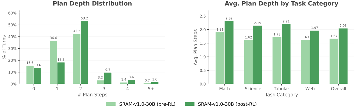
Figure 4: Plan depth analysis of SRAM-v1.0-30B before (light green) and after (green) 200 RL steps. Left: Distribution of plan steps per assistant turn. RL shifts mass from 1-step plans toward 2- and 3+ step plans (5.3% \rightarrow 14.9%), while the proportion of unplanned turns (0 steps) remains stable (15.6% \rightarrow 13.6%), indicating that RL deepens planning without increasing planning frequency. Right: Average plan depth by task category, conditional on planning. All categories show consistent increases, with the largest gain in science (32.7%) and the smallest in web (20.9%), consistent with the latter’s shorter feasible horizon under environmental uncertainty.
