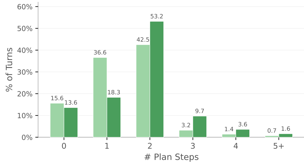
Plan Depth Distribution
