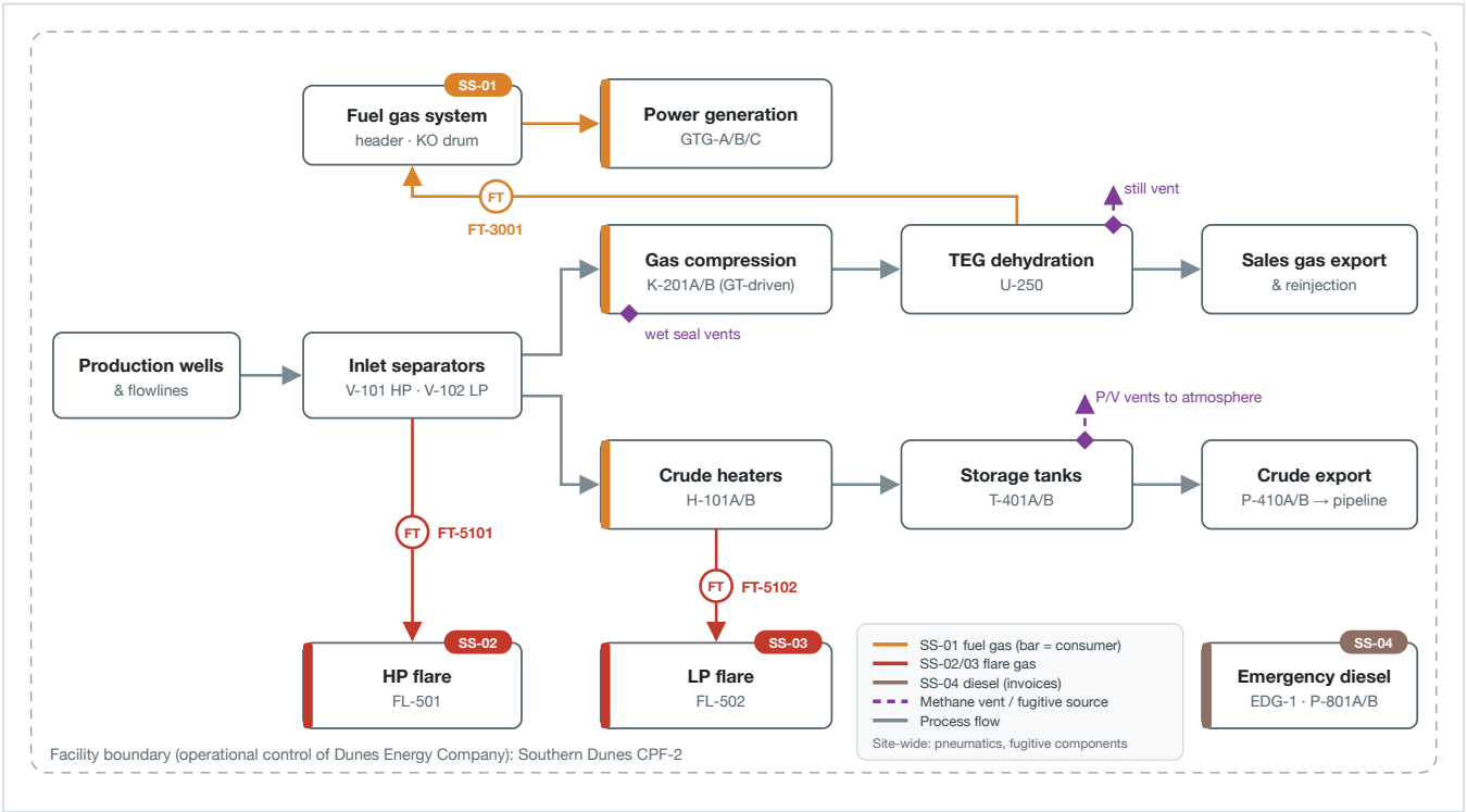
Figure 1: Emission sources, source streams and measurement points at Southern Dunes CPF-2. Tags are referenced throughout this plan and the emissions report.
