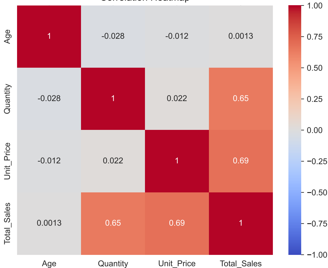
Correlation Heatmap
