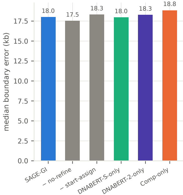
Boundary accuracy
