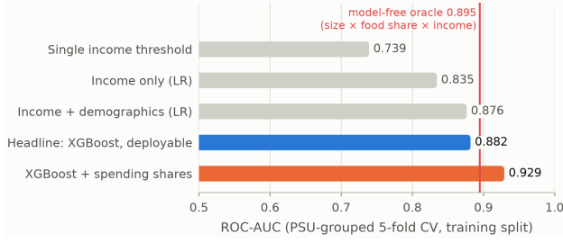
Fig. 1. Grouped-CV ROC-AUC on the training split as features and capacity are added. The red line is the score from household size, food share and income, with no fitted model: it beats every model that does not see spending shares, and the full model’s extra 0.047 AUC over the headline runs largely through that route.
