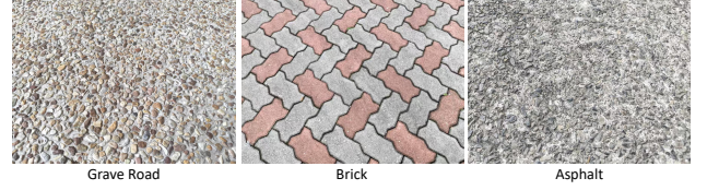
Fig. 5: Examples of the rough ground surfaces used to evaluate robustness against out-of-plane disturbances.
