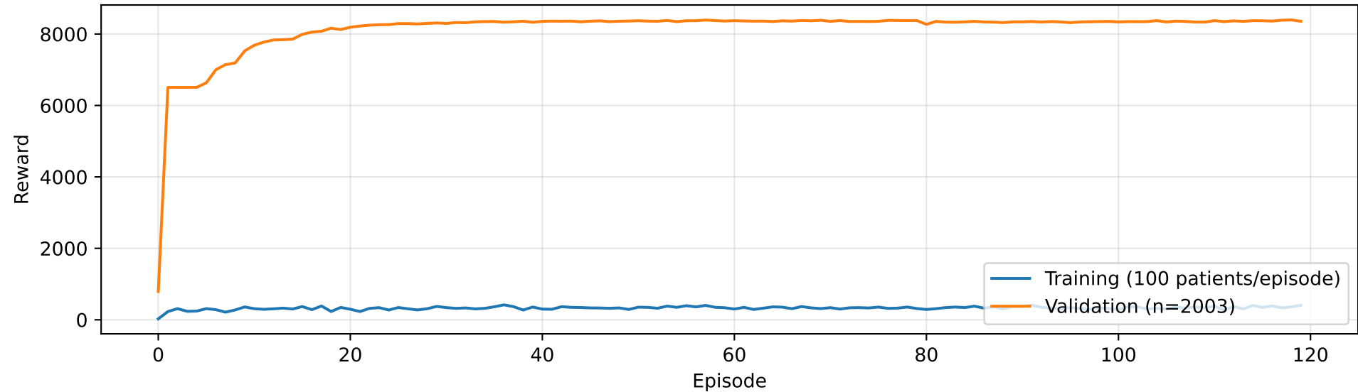
RL DQN reward over training
