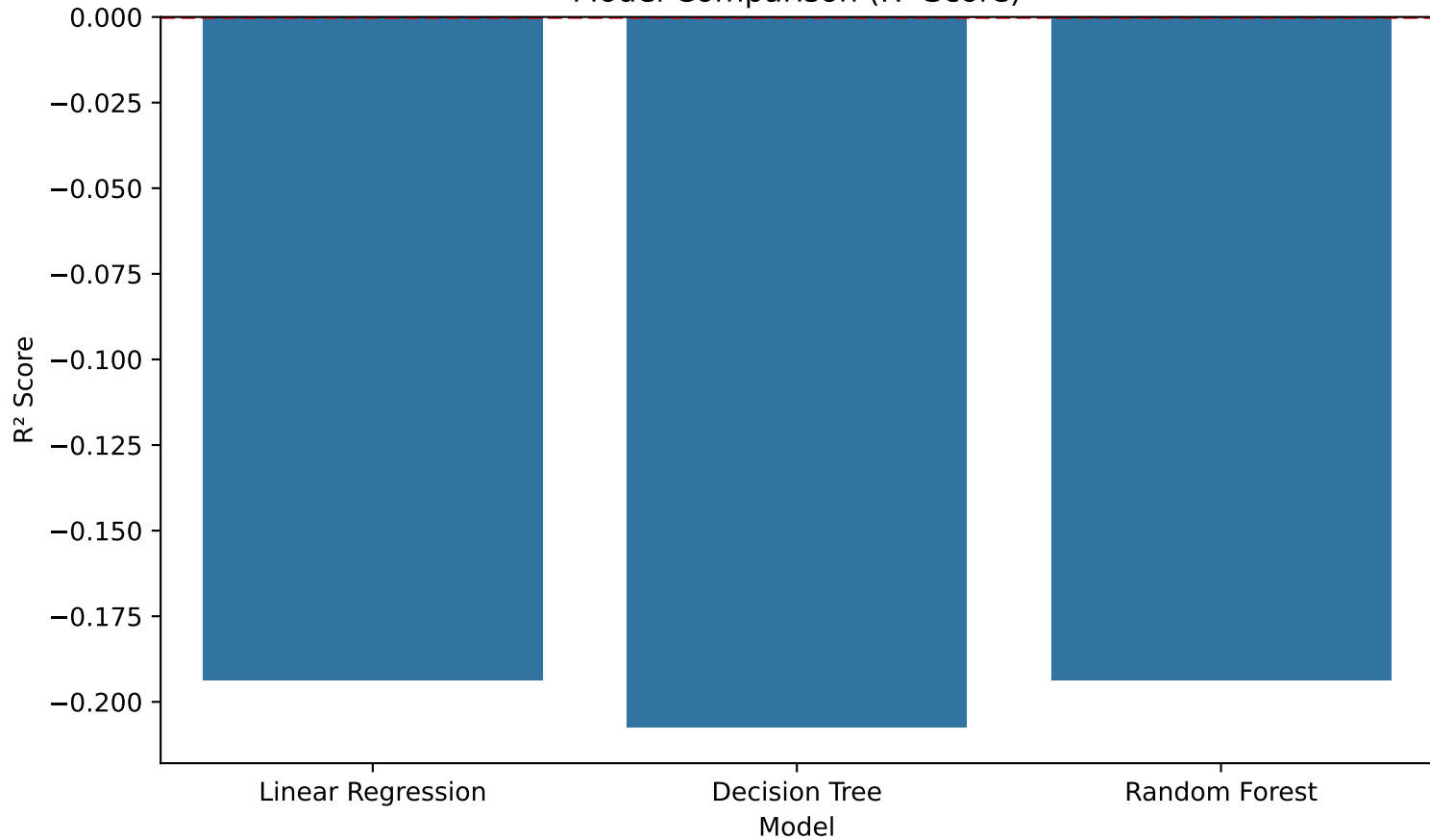
Model Comparison ( R^2 Score)
