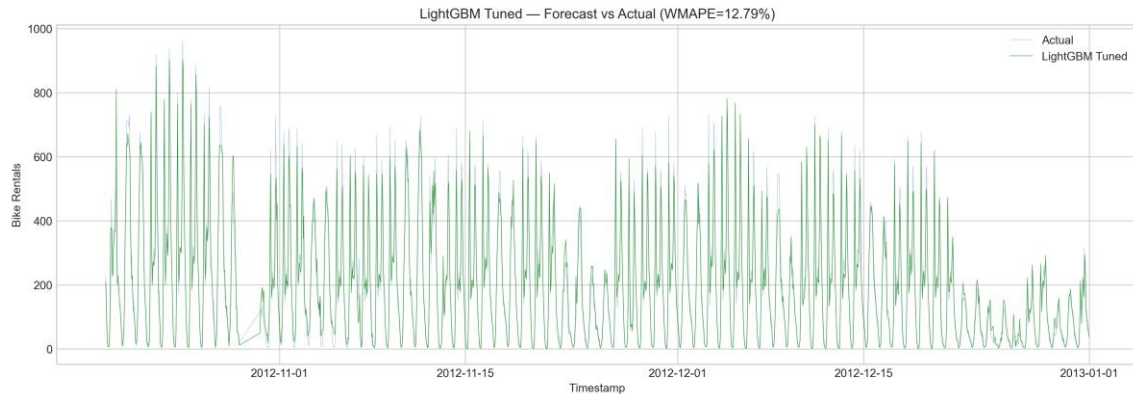
Figure 9: LightGBM Tuned Forecast vs Actual
