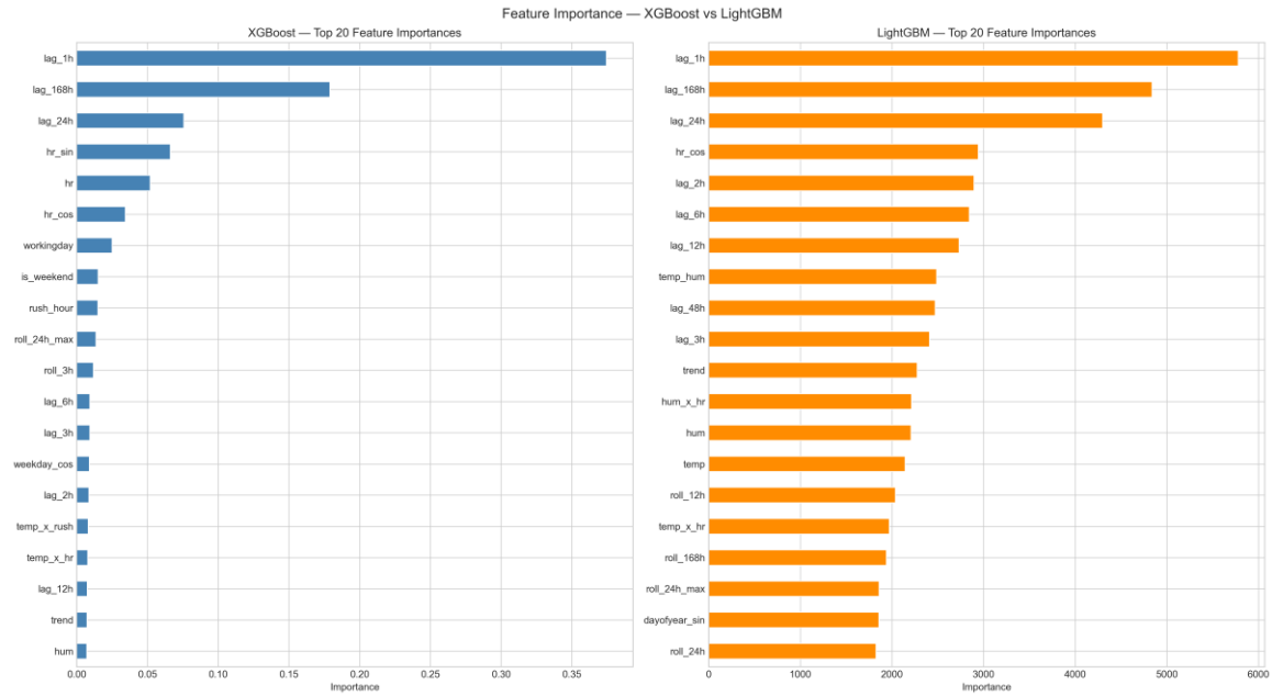
Figure 13: Feature Importance — XGBoost vs LightGBM
