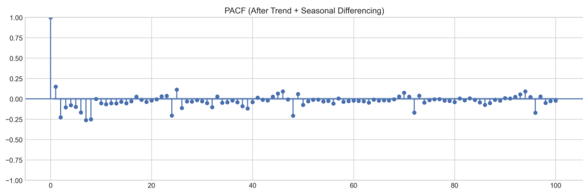
Figure 5: PACF After Trend + Seasonal Differencing
