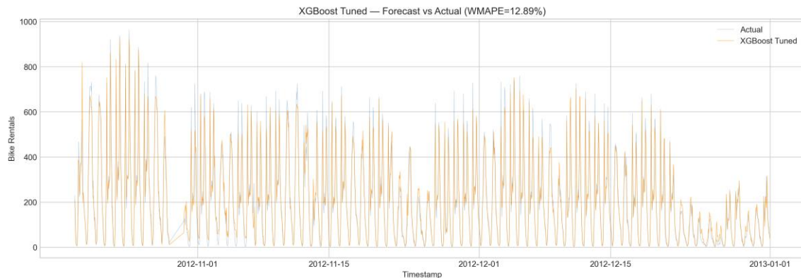
Figure 8: XGBoost Tuned Forecast vs Actual
