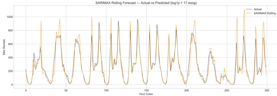
Figure 7: SARIMAX Rolling Forecast vs Actual
