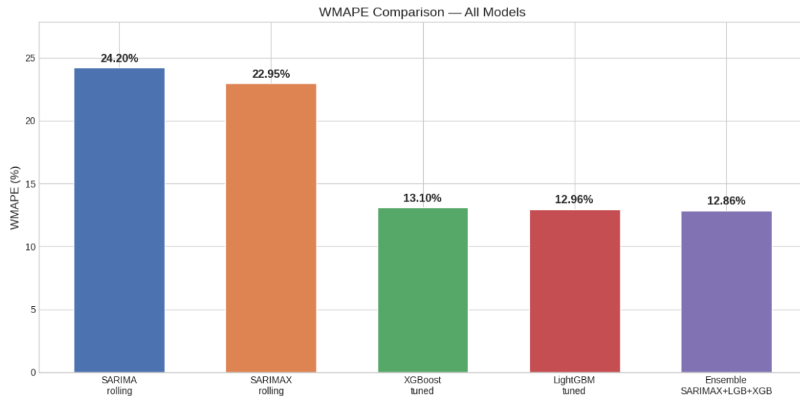
Figure 12: Model Comparison — WMAPE (Lower is Better)
