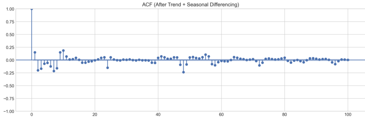
Figure 4: ACF After Trend + Seasonal Differencing
