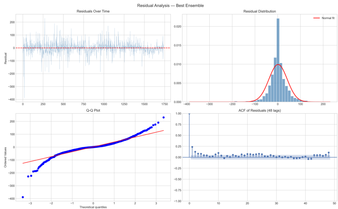
Figure 20: Residual Analysis — Best Ensemble
