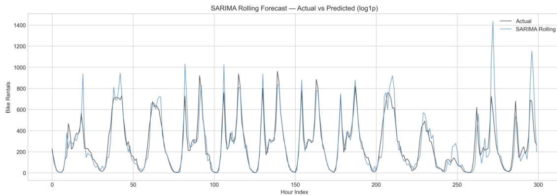
Figure 6: SARIMA Rolling Forecast vs Actual
