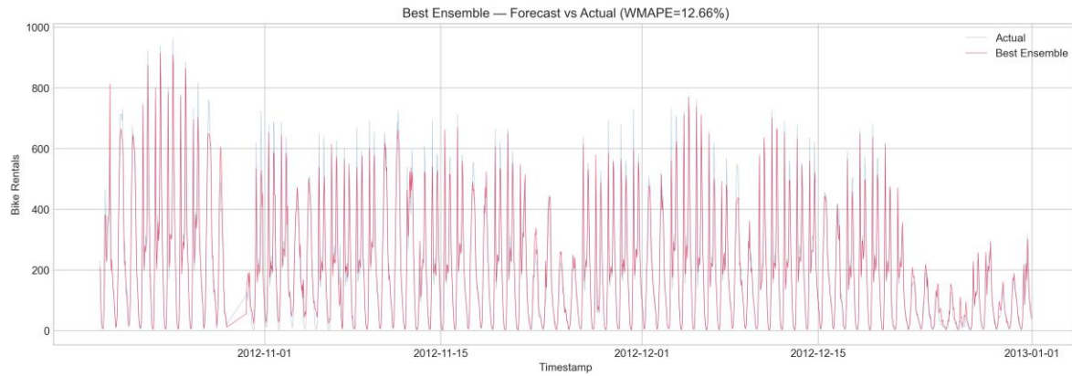
Figure 11: Best Ensemble Forecast vs Actual
