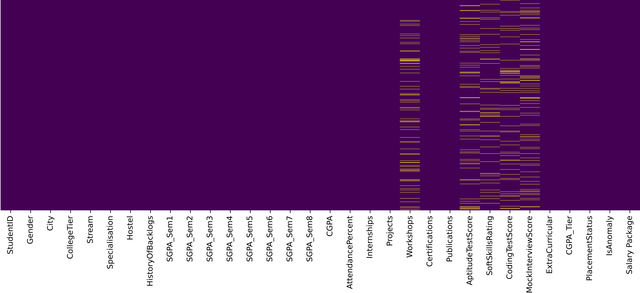
Missing Value Heatmap
