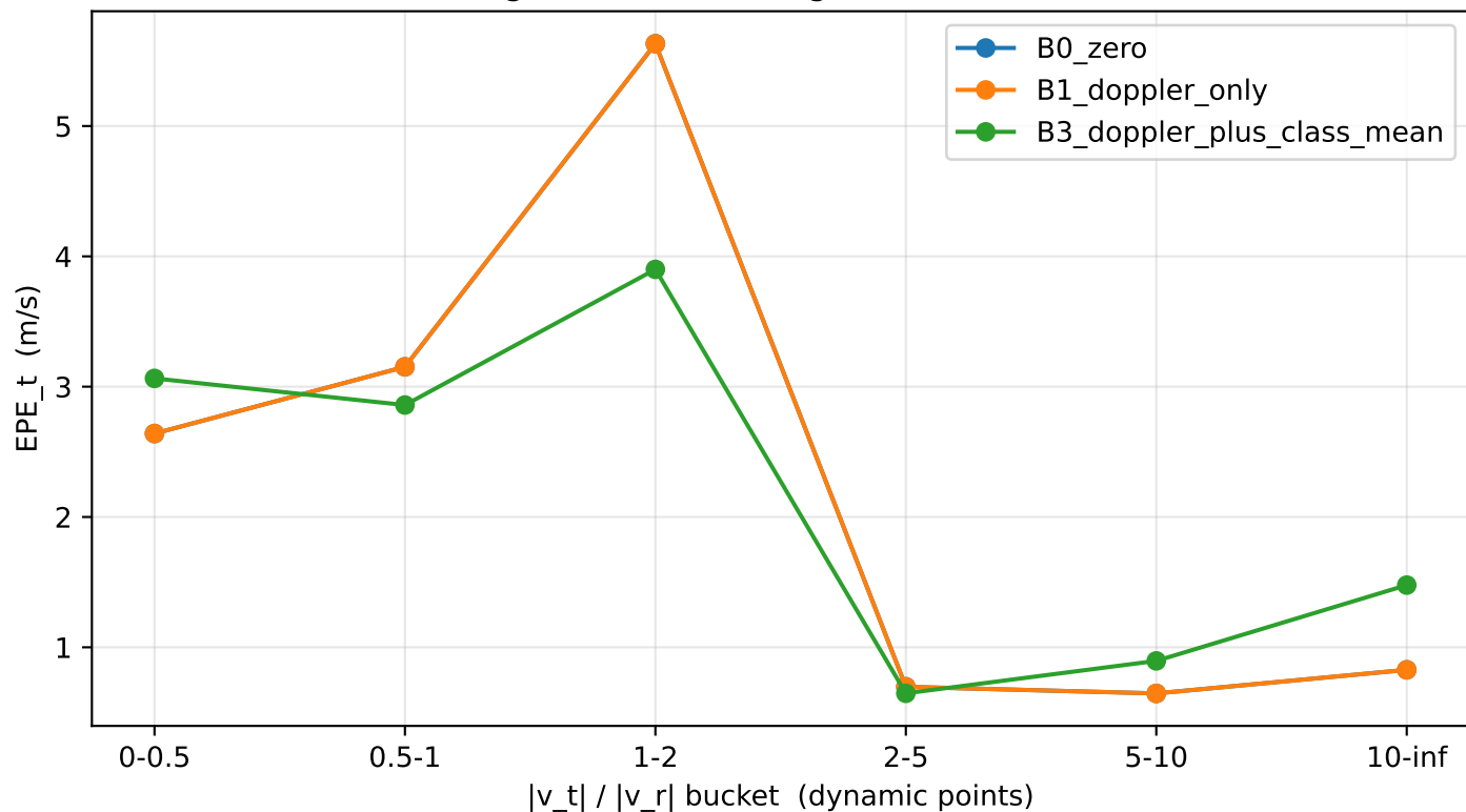
F3 — Tangential EPE vs tangential-dominance ratio
