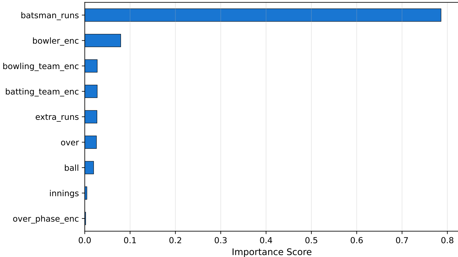
Figure 2.3 — Random Forest Feature Importances (Including Bowler Identity)
