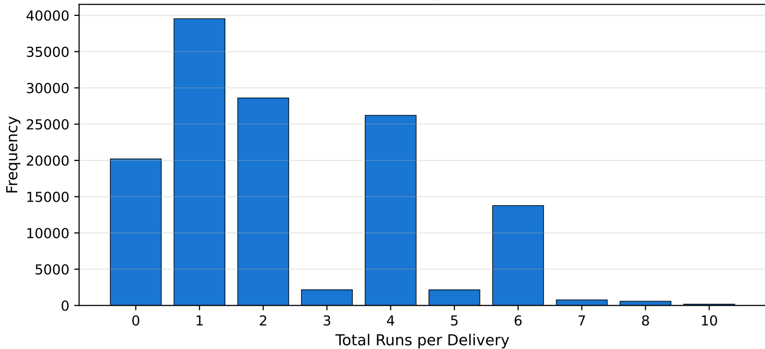
Distribution of total_runs per Delivery
