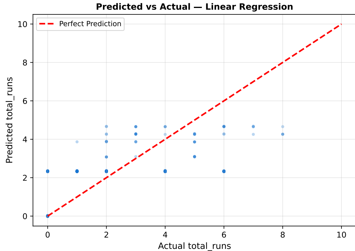
Figure 4.1 — Regression Results: Linear Regression
