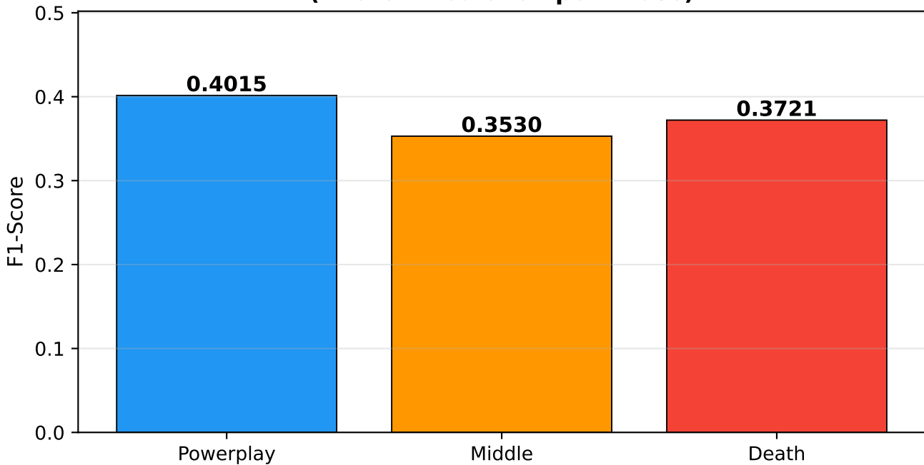
Figure 5.2 — Phase-Specific Model F1-Scores (Wicket Prediction per Phase)
