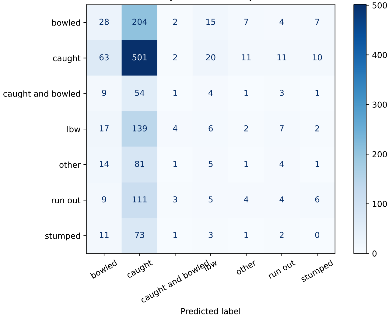
Figure 6.1 — Confusion Matrix: Dismissal Type Classification (Random Forest)
