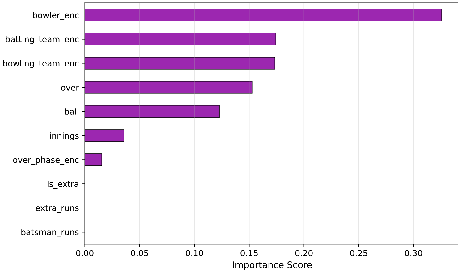
Figure 6.2 — Feature Importances for Dismissal Type Classification
