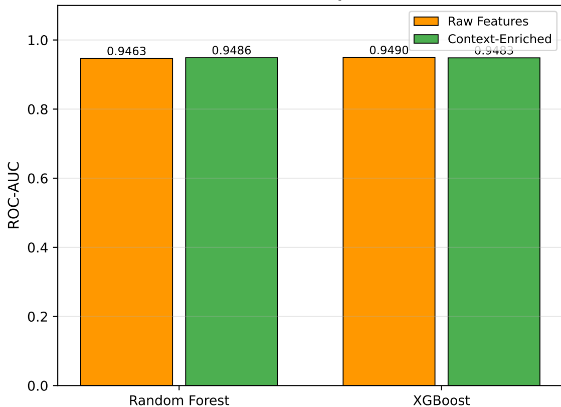
ROC-AUC Comparison
