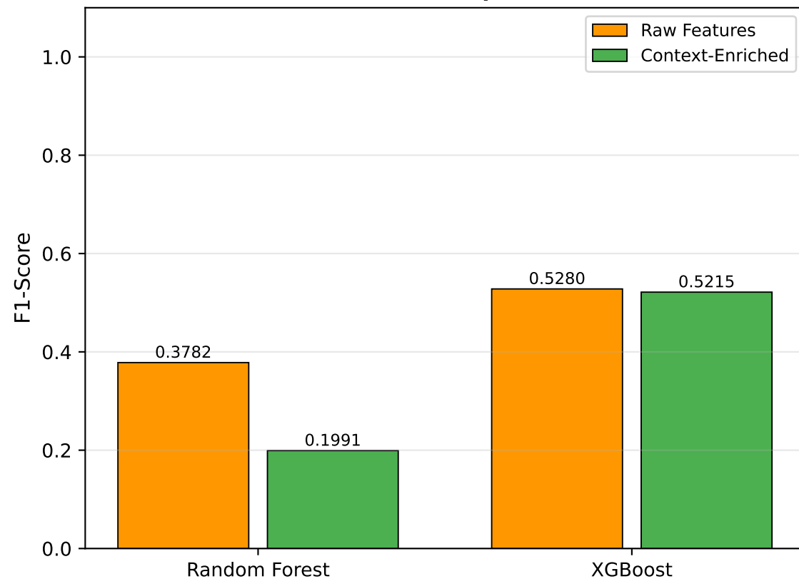
F1-Score Comparison
