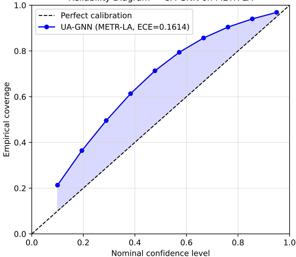
Reliability Diagram — UA-GNN on METR-LA
