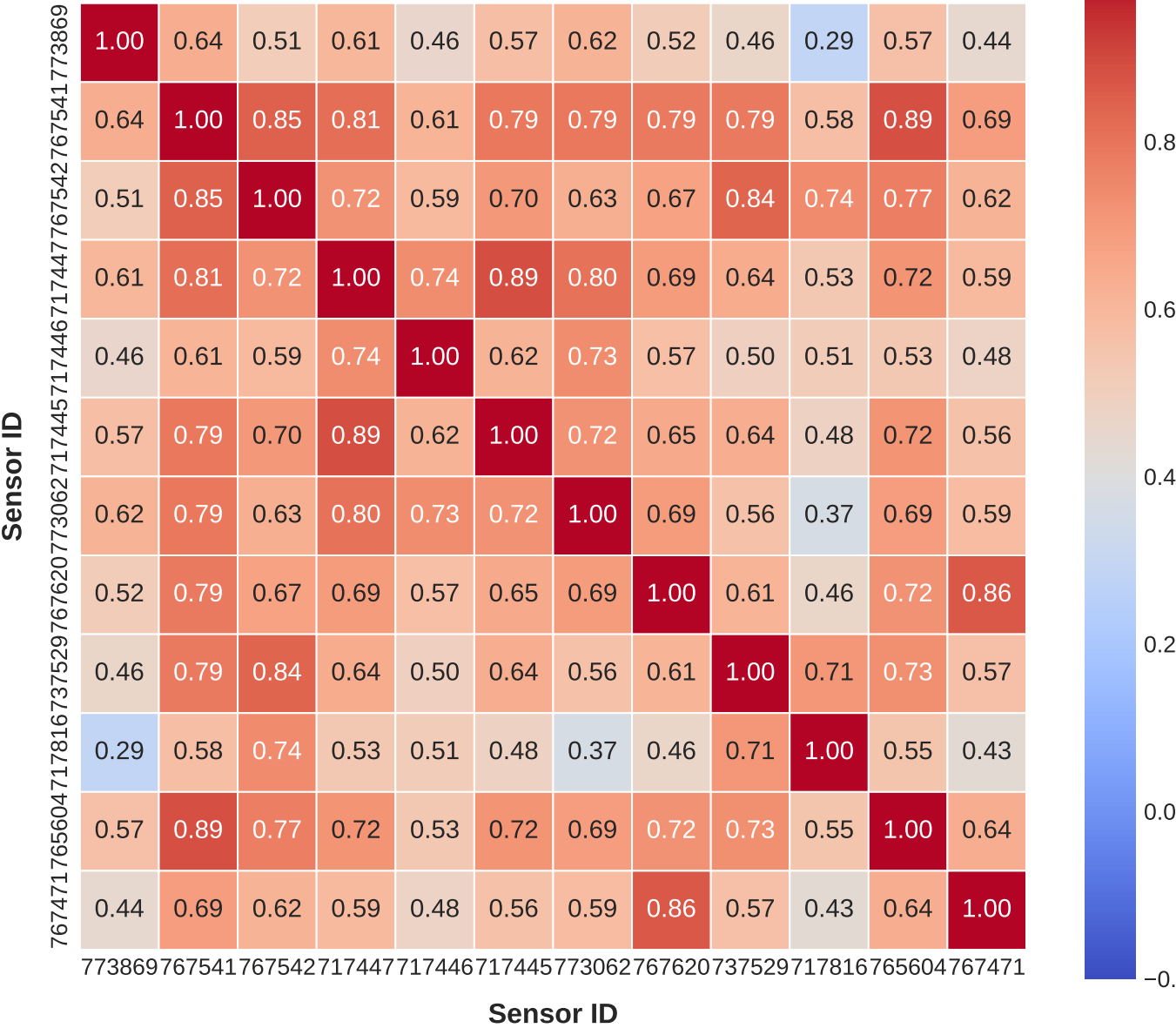
Spatial Correlation Matrix for METR-LA Sensor Subset (Motivating Graph-Based Spatial Modeling)
