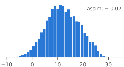
log(1 + Evaporation)
