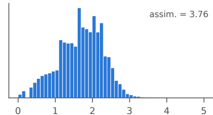
Humidity3pm
