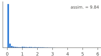
WindGustSpeed
