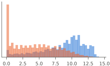
WindGustSpeed
