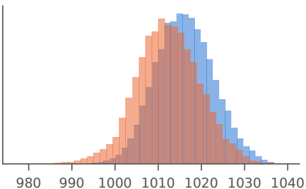
Pressure3pm
