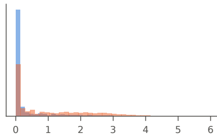
log(1 + Rainfall)
