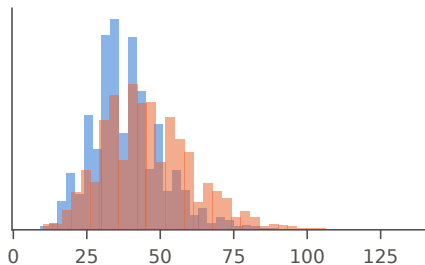
WindGustSpeed
