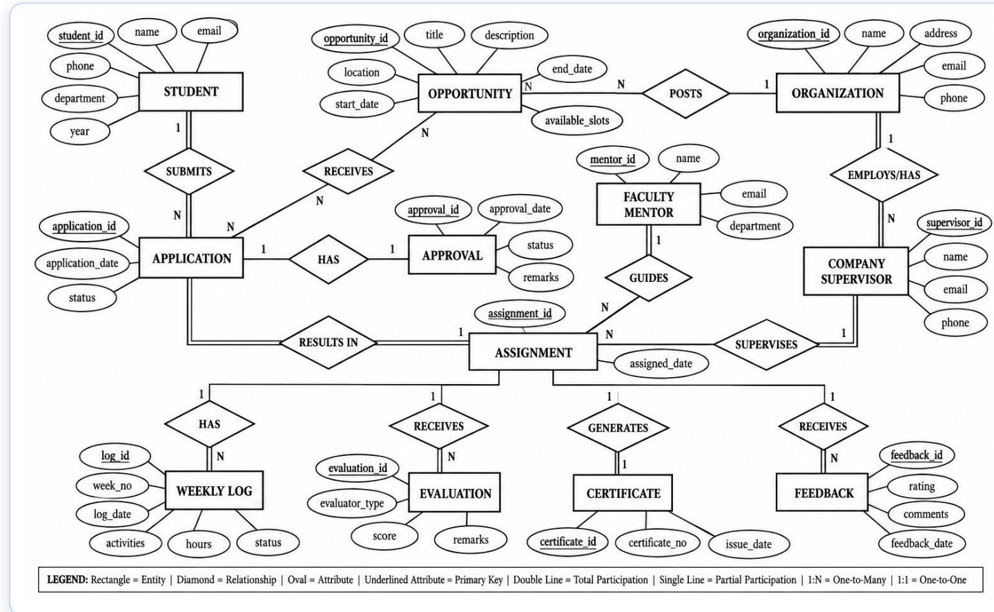
Final ER diagram (report, Figure 2)
