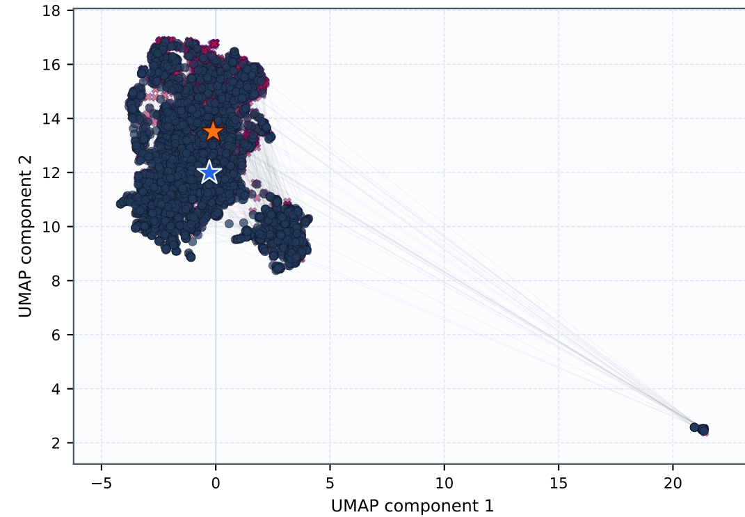
Human-HDPO Centroid distance: 1.531
