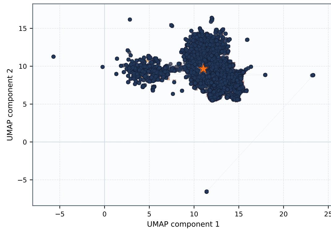
Human-FullSFT Centroid distance: 0.018
