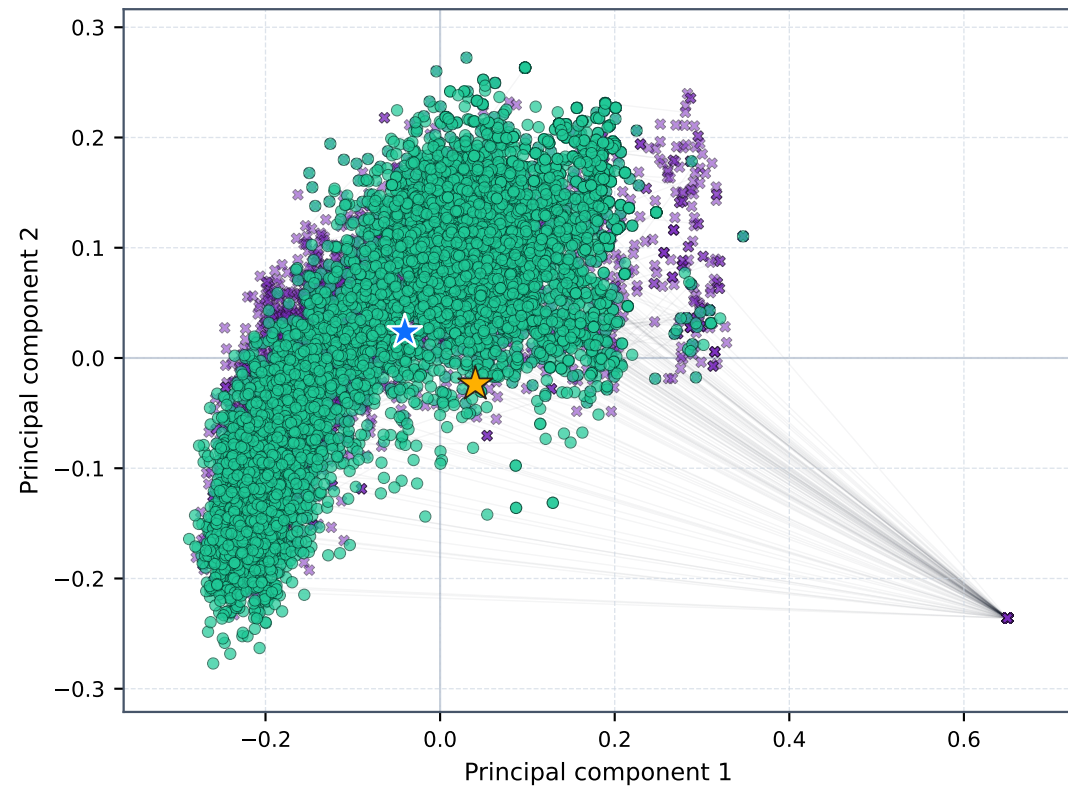
test-baselm (n=6357)
