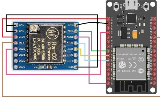
Fig. 4: Pin configuration
