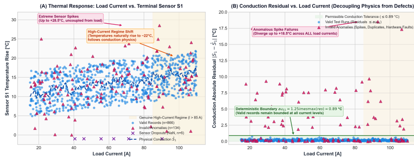
Figure 1: High operating load ( I > 85^\circ\text{A} ) follows the deterministic physical heating curve rather than an anomaly, whereas true anomalies (sensor spikes, dropouts, duplicates) are scattered completely independent of load level.
