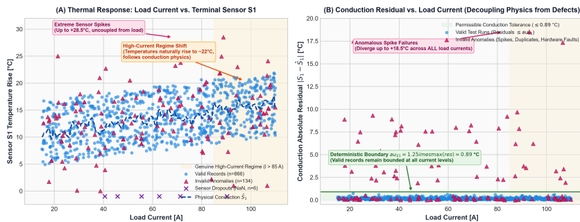
Figure 1: High operating load ( I > 85 A) follows the deterministic physical heating curve rather than an anomaly, whereas true anomalies (sensor spikes, dropouts, duplicates) are scattered completely independent of load level.
