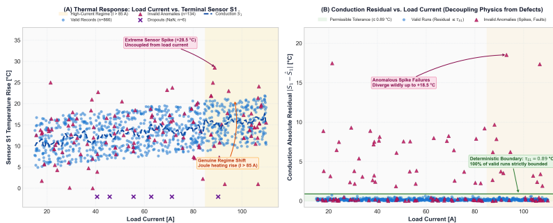
Figure 1: High operating load ( I > 85 A) follows the deterministic physical heating curve rather than an anomaly, whereas true anomalies (sensor spikes, dropouts, duplicates) are scattered completely independent of load level.
