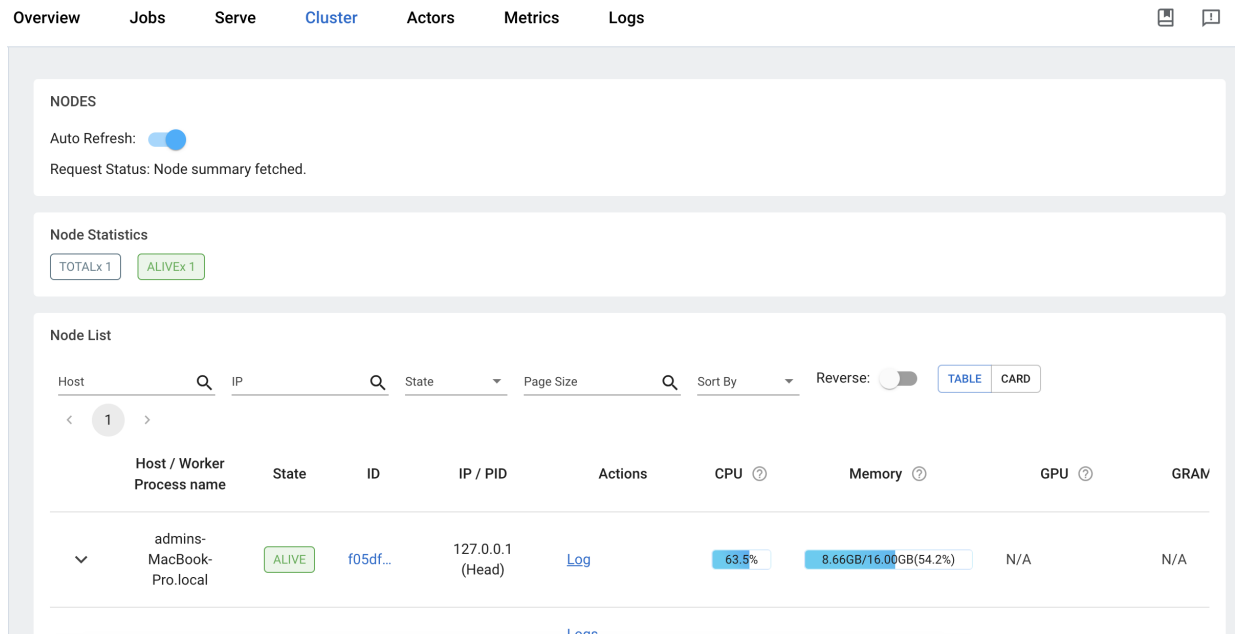
Figure 9.4: Ray Dashboard.
