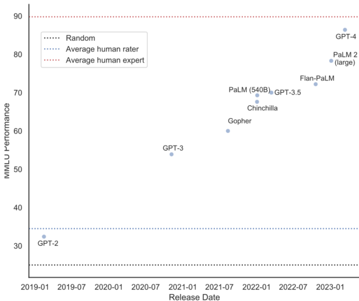
Figure 1.1: Average performance on the Massive Multitask Language Understanding (MMLU) benchmark of Large Language Models (LLM). Please note that while most benchmark results come from 5-shot, a few the GPT-2, PaLM, and PaLM-2 results refer to fine-tuned models.
