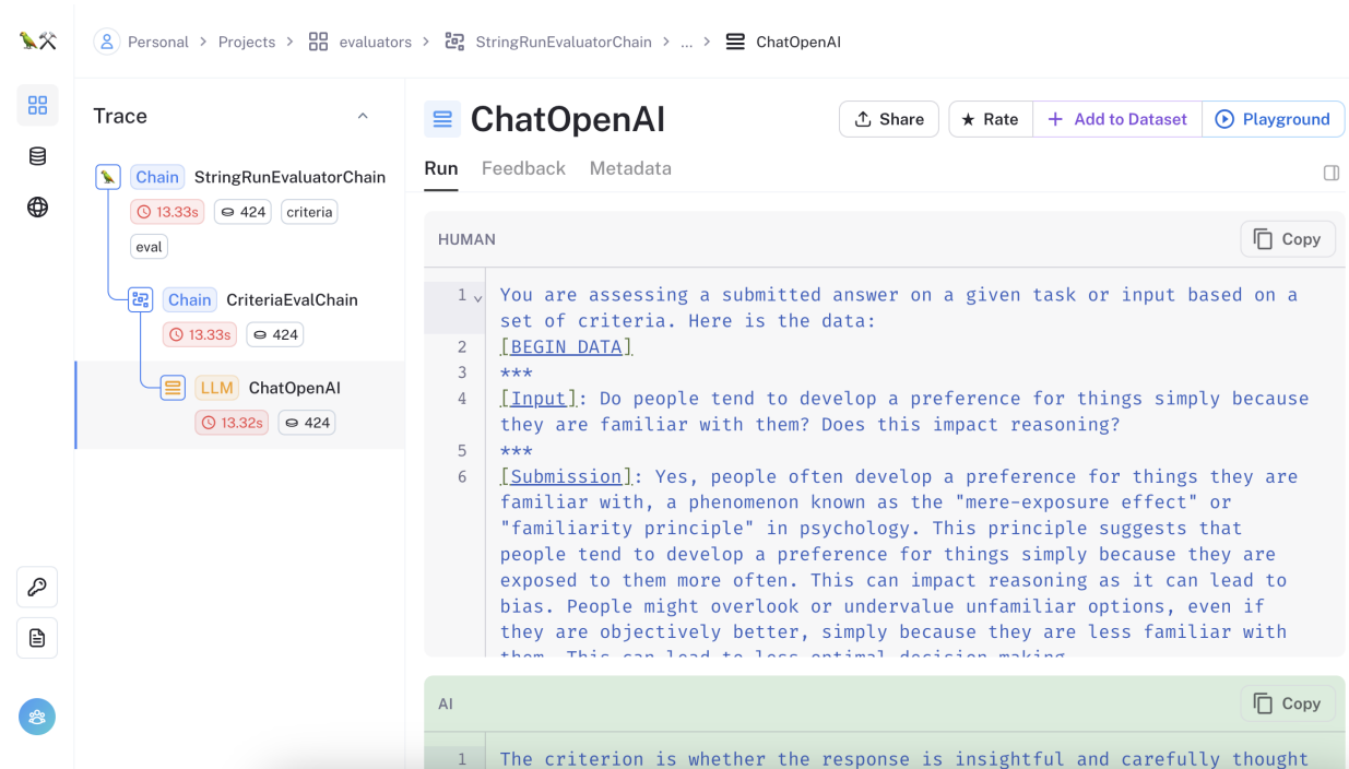
Figure 9.7: Tracing in LangSmith.
