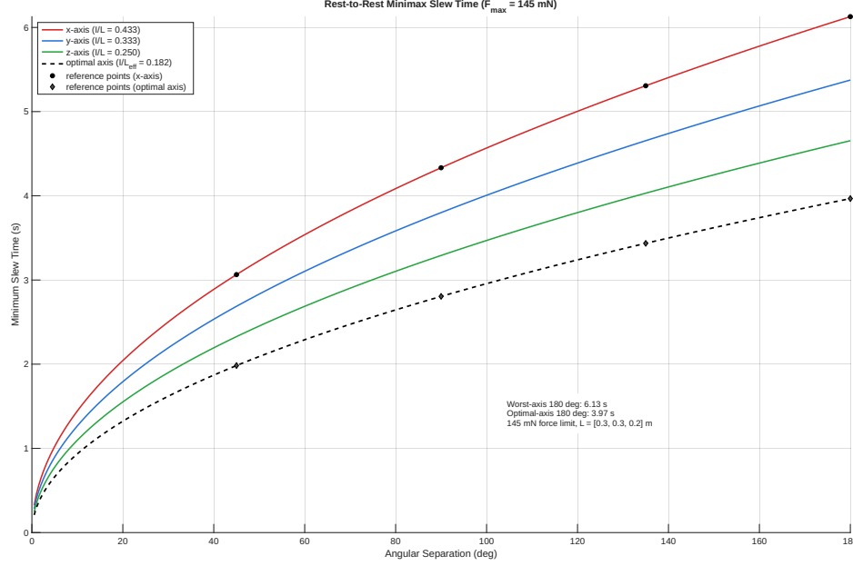
Fig. 2 Force-limited minimum slew time versus angular separation for the 12 kg 6U reference vehicle. The 145 mN force budget permits sub-7 s rest-to-rest slews even for a worst-axis 180° maneuver.
