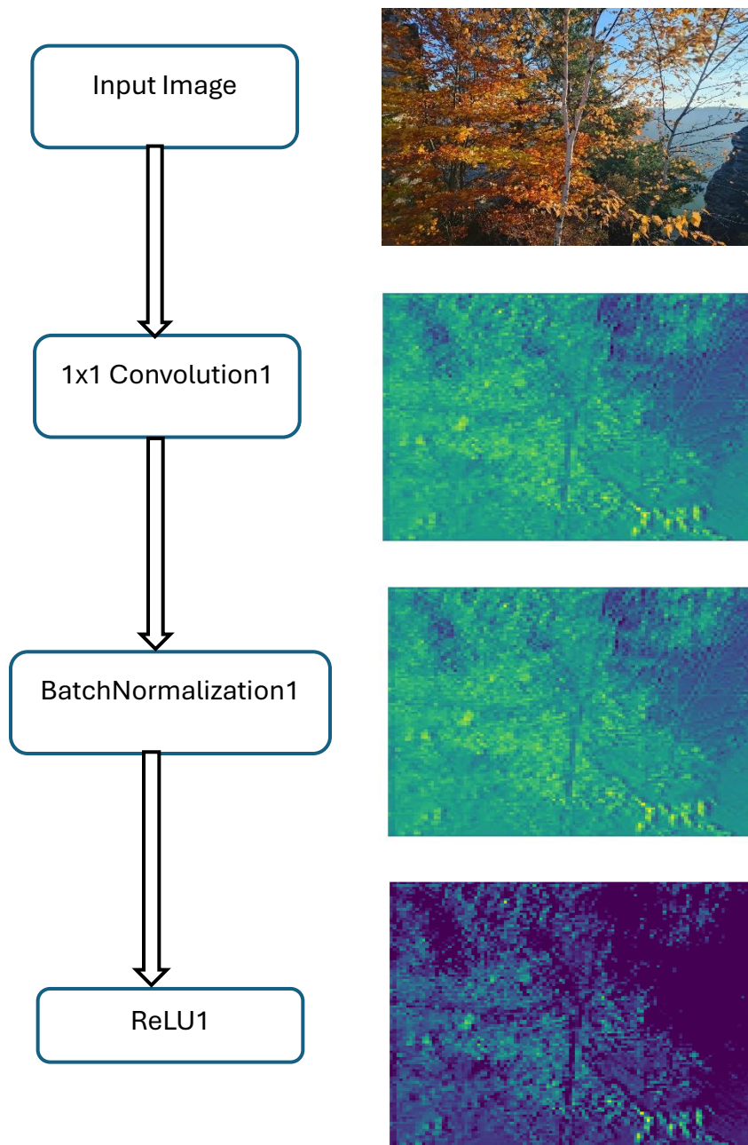
Figure 6: Flowchart indicating transformation of images during single convolutional layer of Bottleneck block after each step of convolution layer (Convolution1, Batch Normalization, ReLU). The images show only the first feature map of the first channel after each convolution step to simplify the visualization.
