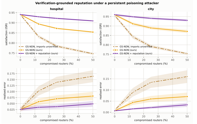
Fig. 2. Satisfaction and realised error under a persistent poisoning attacker. Reputation is free at zero compromise and recovers most of the attack’s cost thereafter.
