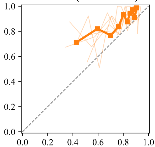
SurvPath (1-cal: 5/5 fail)
