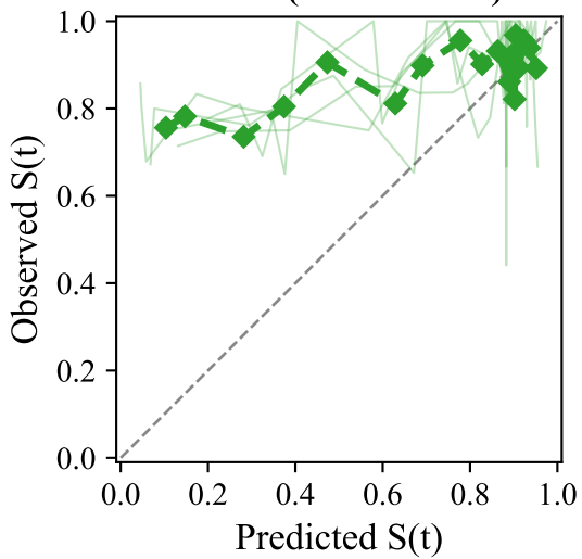
MCAT (1-cal: 5/5 fail)
