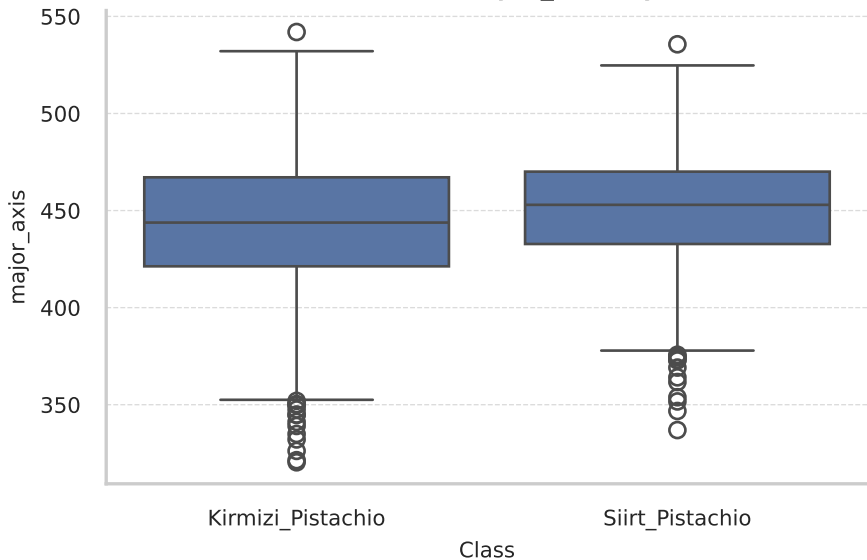
Distribution of major_axis by Class
