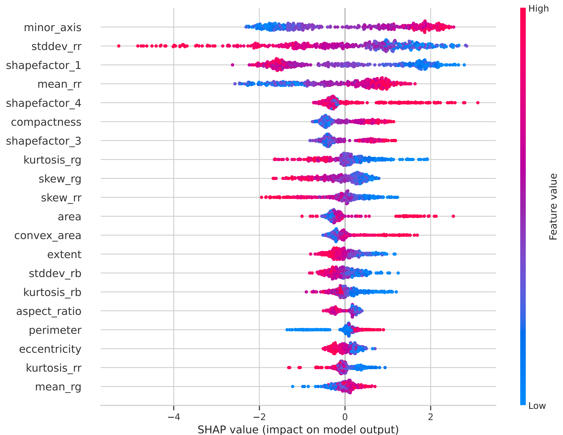
SHAP Feature Importance for Class "Siirt_Pistachio" - LightGBM
