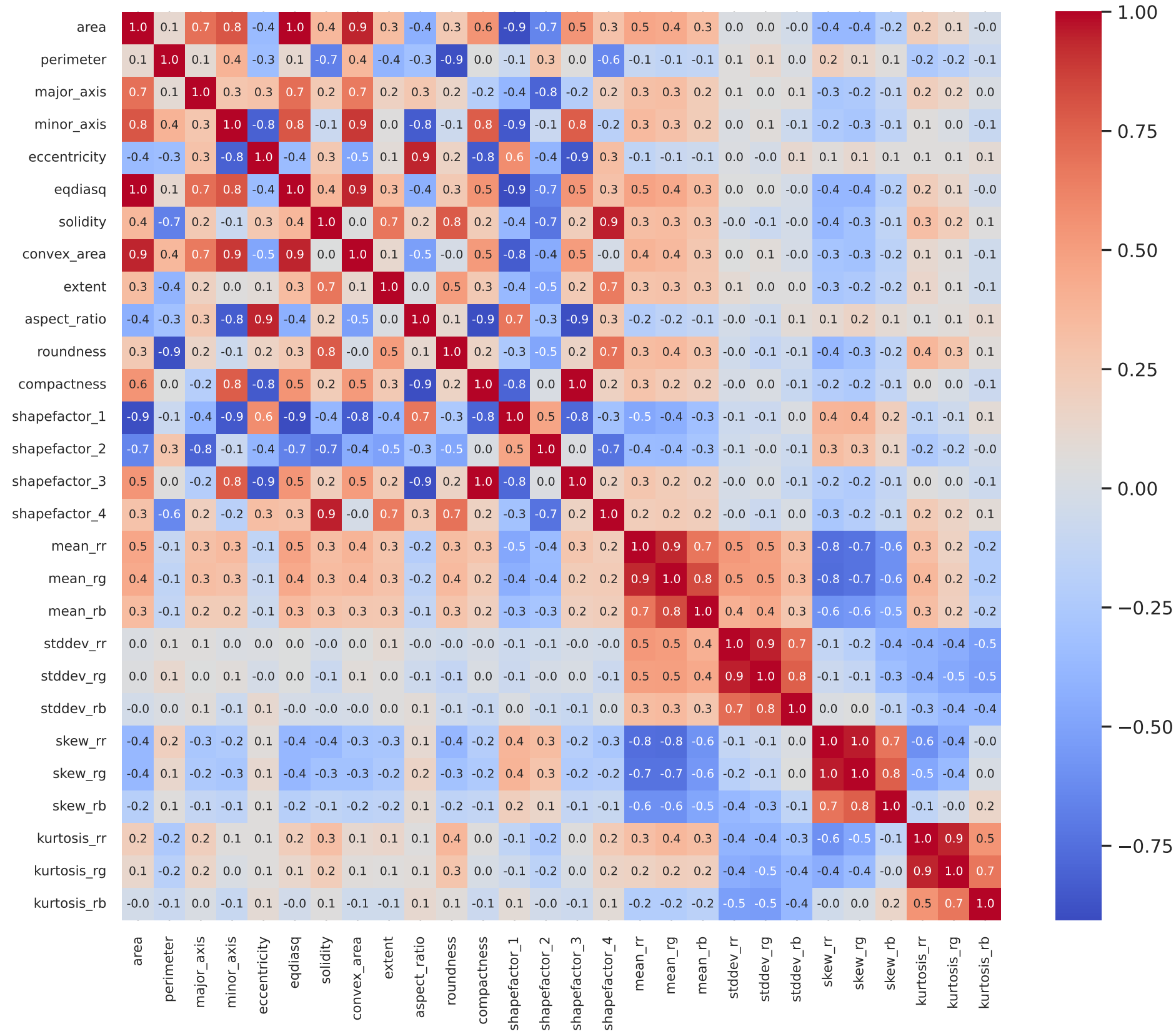
Correlation Matrix of Numeric Features
