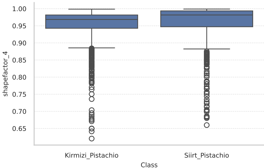
Distribution of shapefactor_4 by Class
