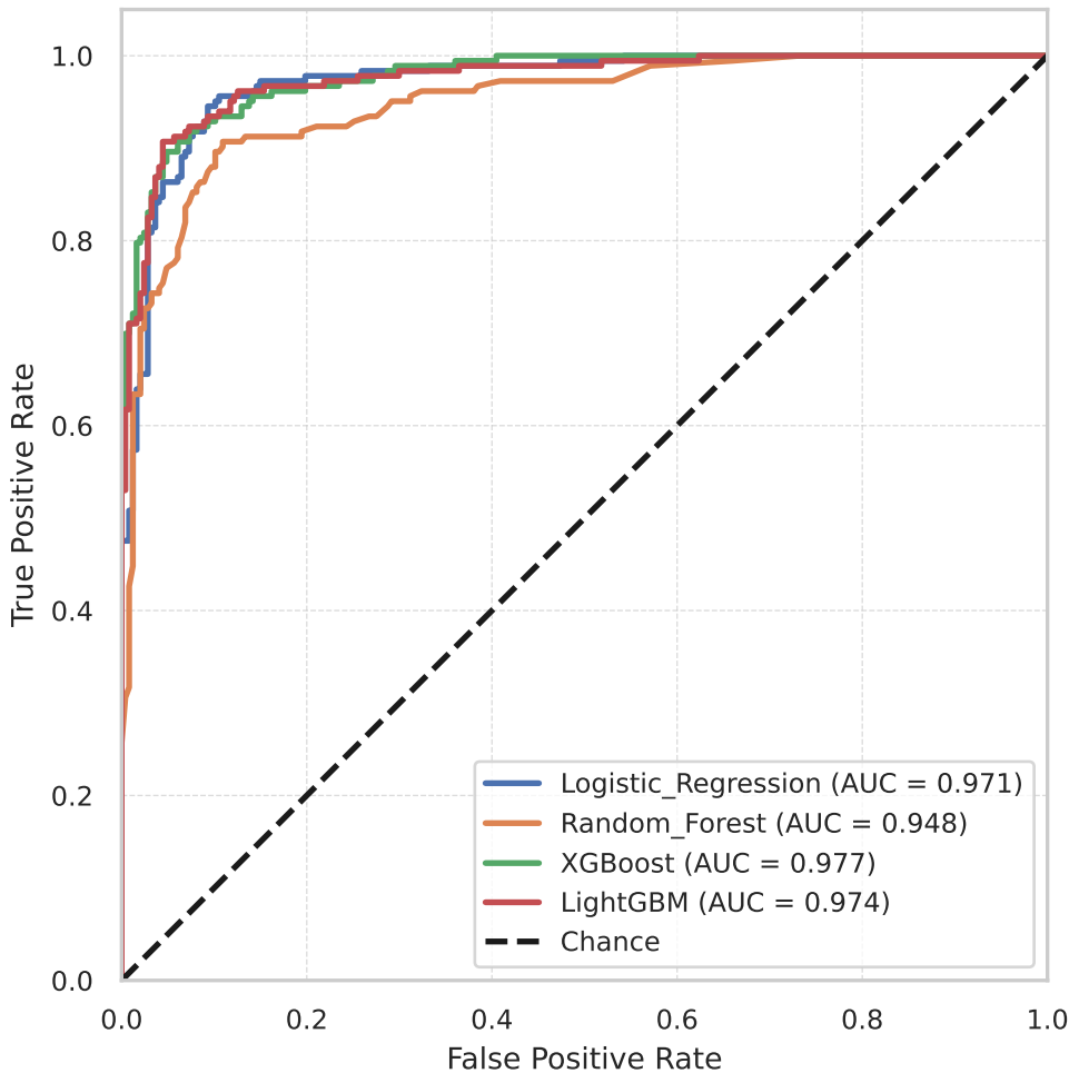
Comparative ROC Curves
