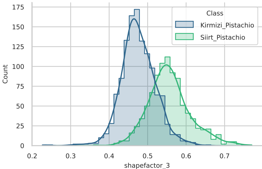
Distribution of shapefactor_3 for each Class
