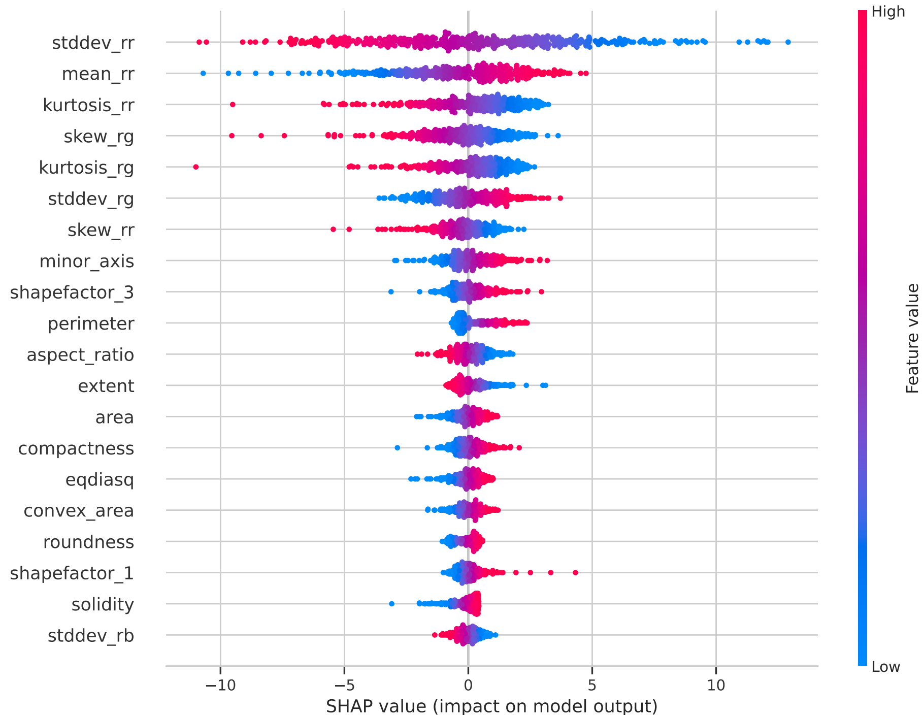
SHAP Feature Importance for Class "Siirt_Pistachio" - Logistic_Regression
