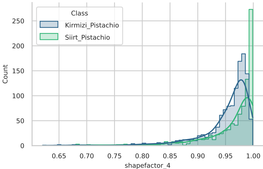
Distribution of shapefactor_4 for each Class
