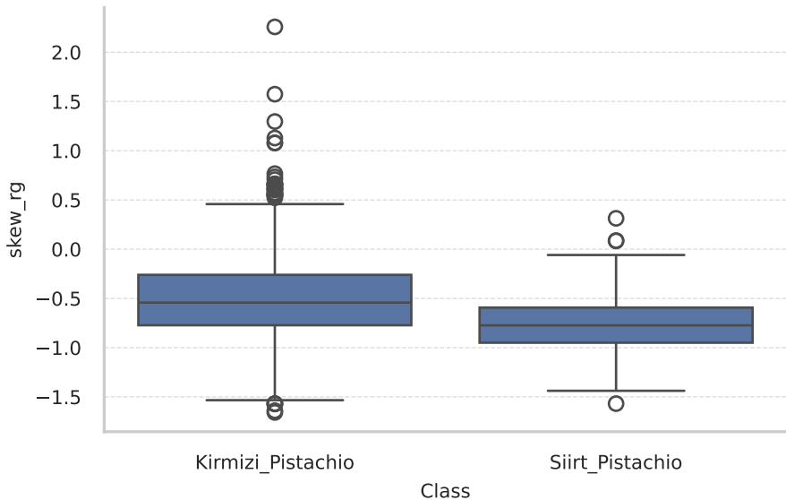
Distribution of skew_rg by Class
