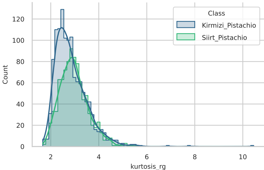
Distribution of kurtosis_rg for each Class
