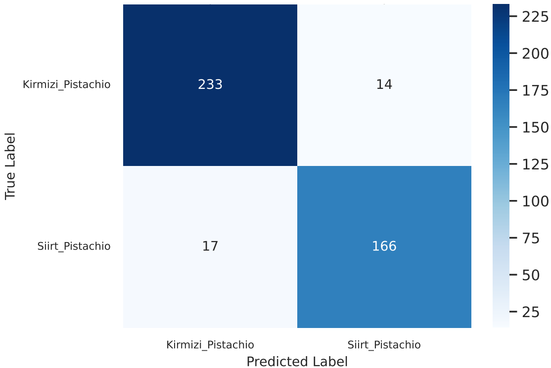
Confusion Matrix - LightGBM
