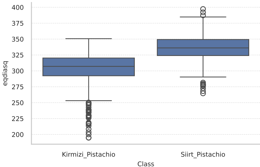
Distribution of eqdiasq by Class
