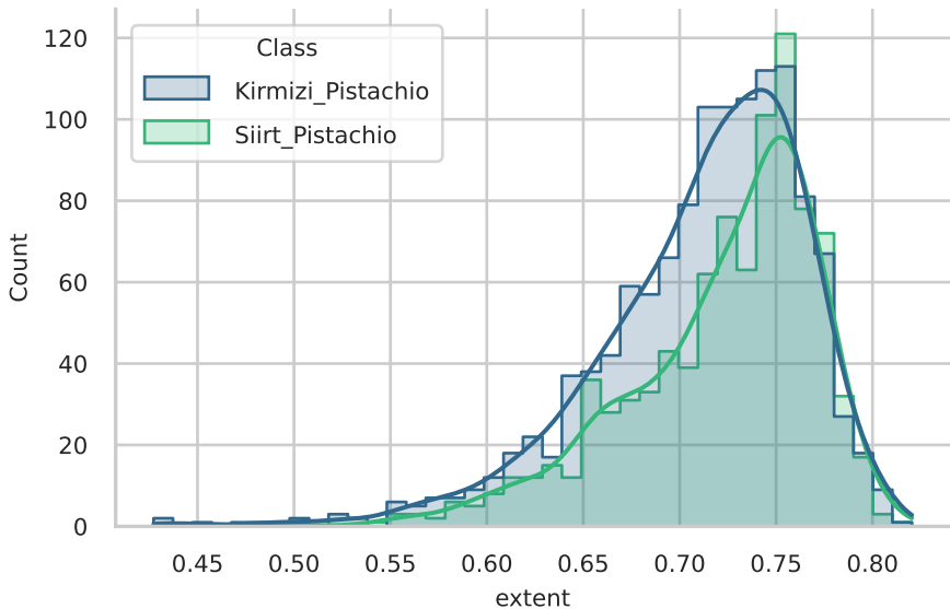
Distribution of extent for each Class
