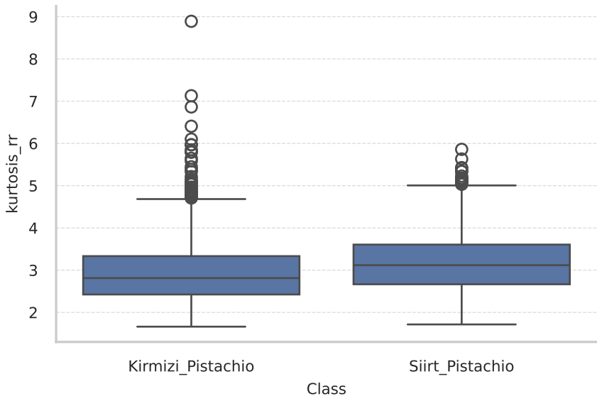
Distribution of kurtosis_rr by Class
