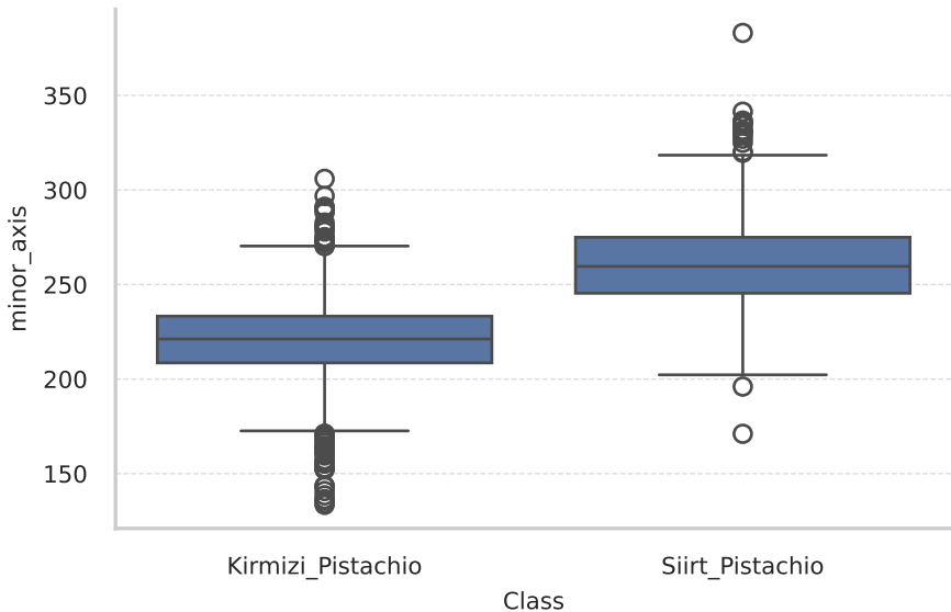
Distribution of minor_axis by Class
