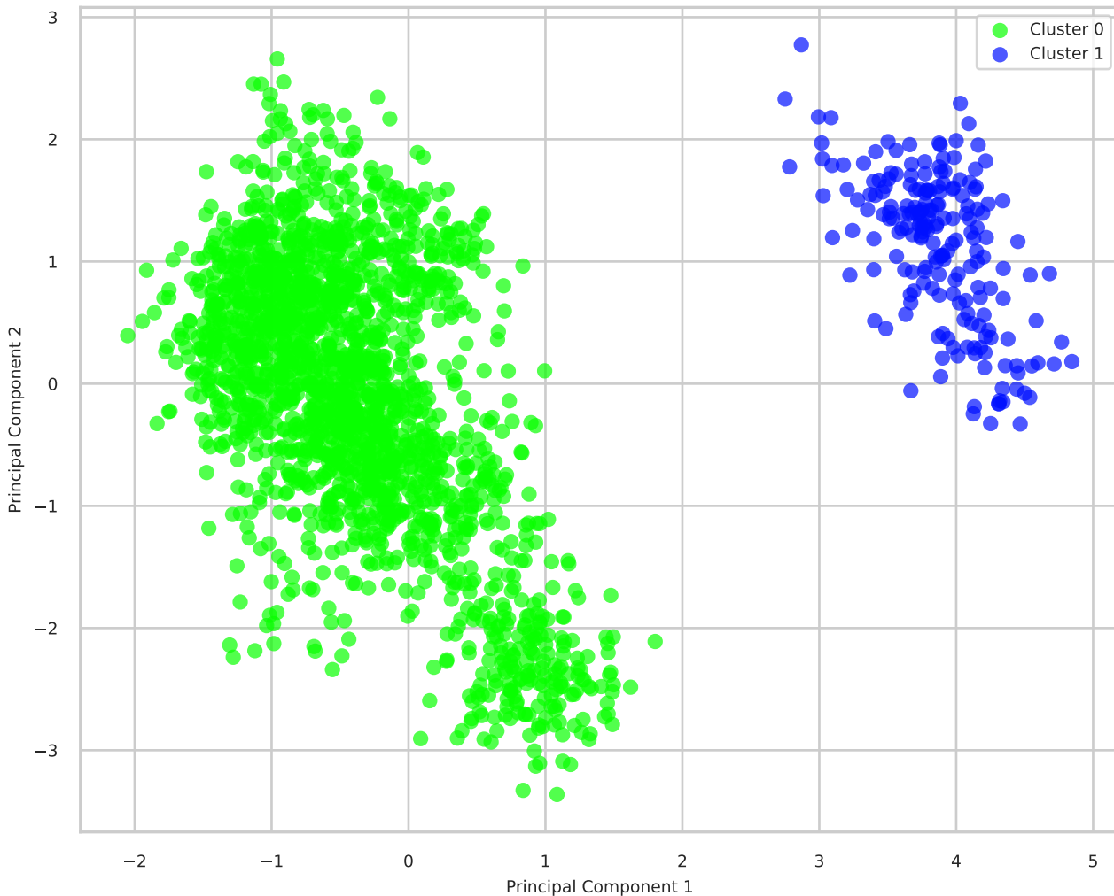
Clusters by Agglomerative on PCA (With_Derived_Features)
