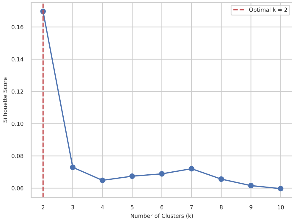
Silhouette Score for KMeans (Original_Features_Only)
