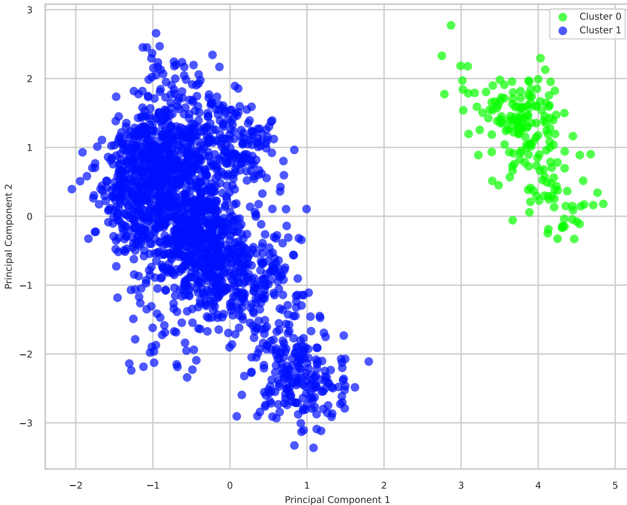
Clusters by KMeans on PCA (Original_Features_Only)
