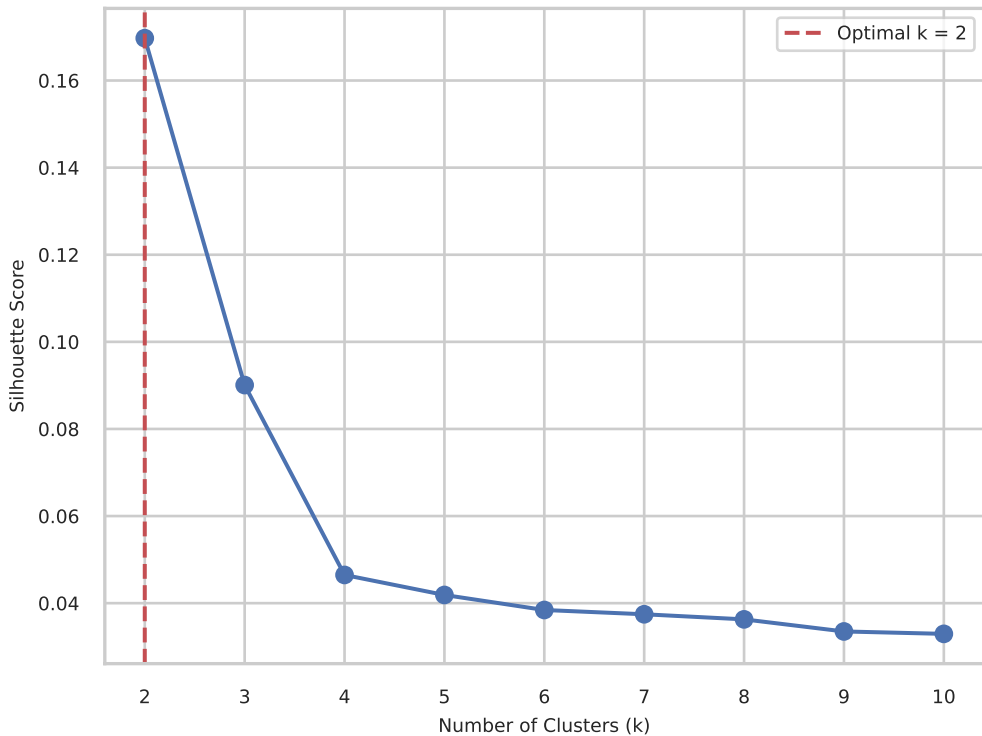
Silhouette Score for Agglomerative (With_Derived_Features)
