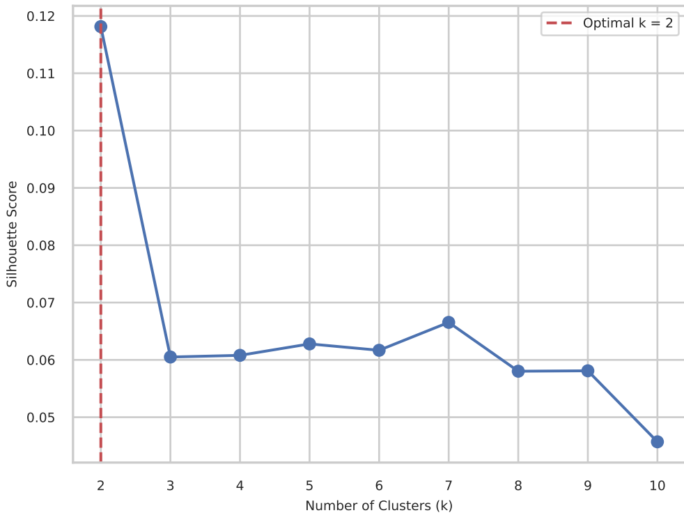
Silhouette Score for GMM (Original_Features_Only)
