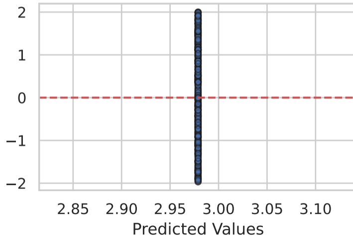
Residuals Analysis
