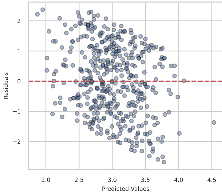
Model Evaluation: SVR Residuals Analysis
