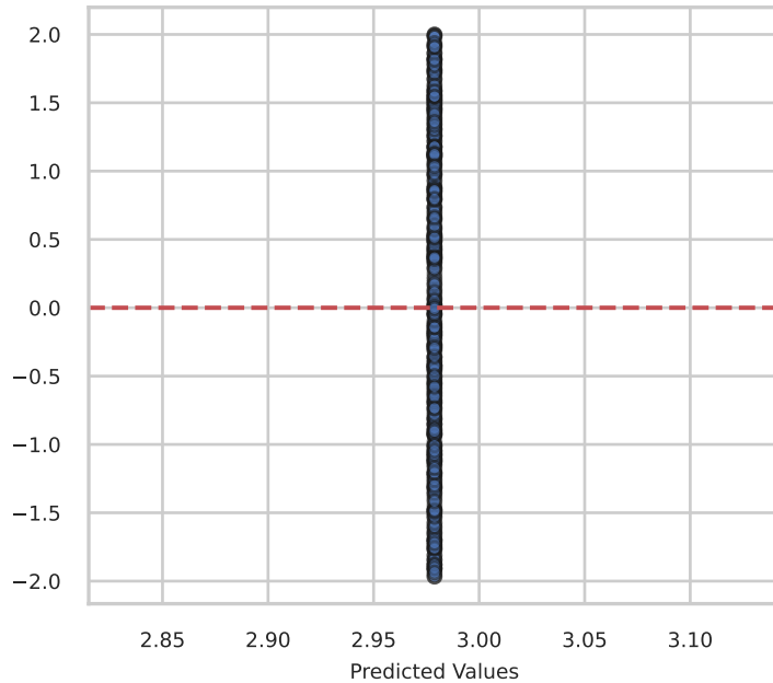
Model Evaluation: Lasso Residuals Analysis
