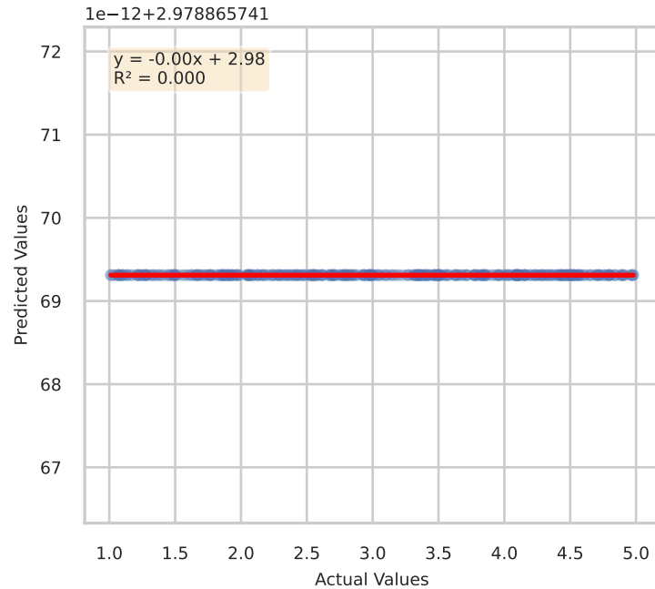
Regression Plot (Seaborn)
