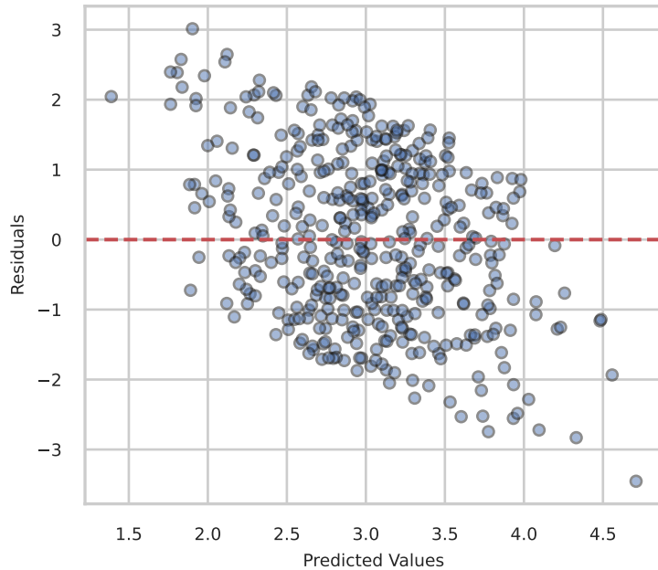
Model Evaluation: XGBoost Regressor Residuals Analysis
