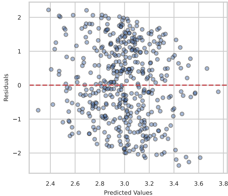
Model Evaluation: Random Forest Regressor Residuals Analysis
