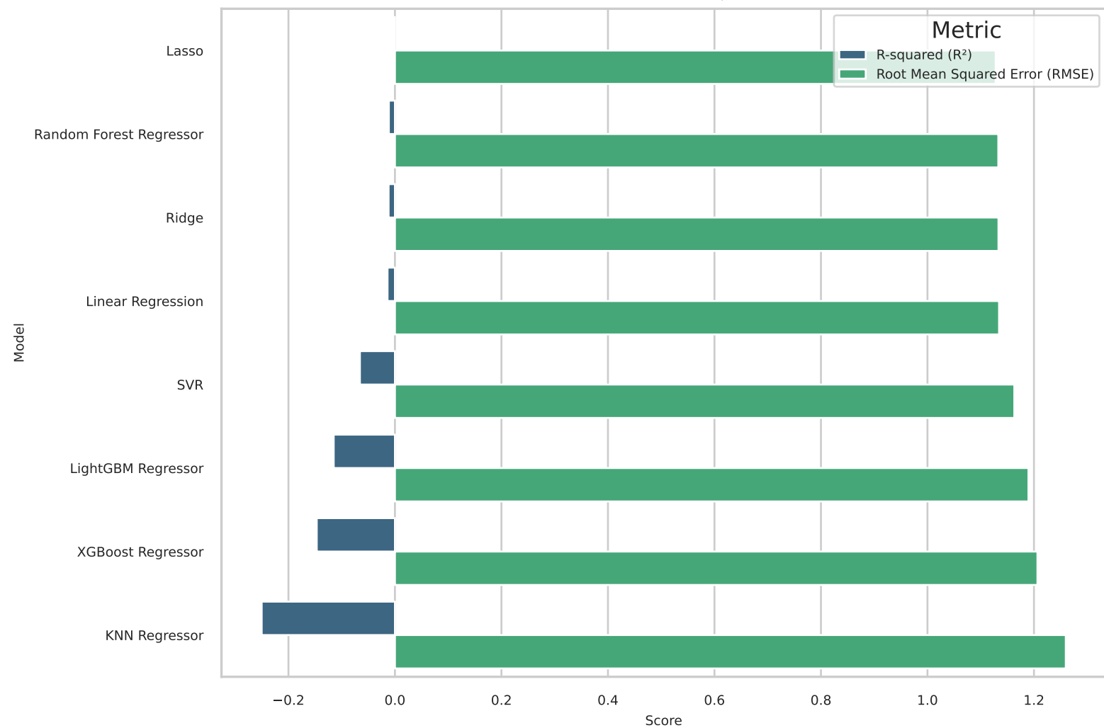
Model Performance Comparison
