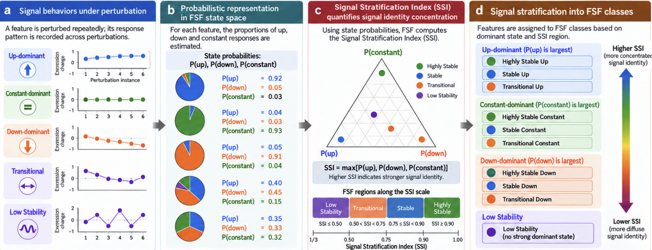
Figure 1. Feature Signal Stratification From perturbation effects to condition-level signal architecture
