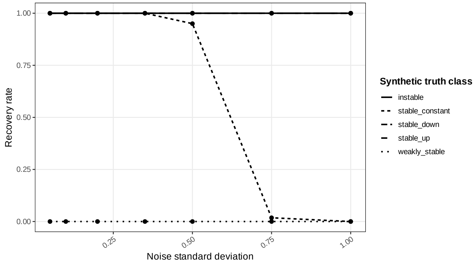
Figure 6C. Synthetic class recovery across noise
