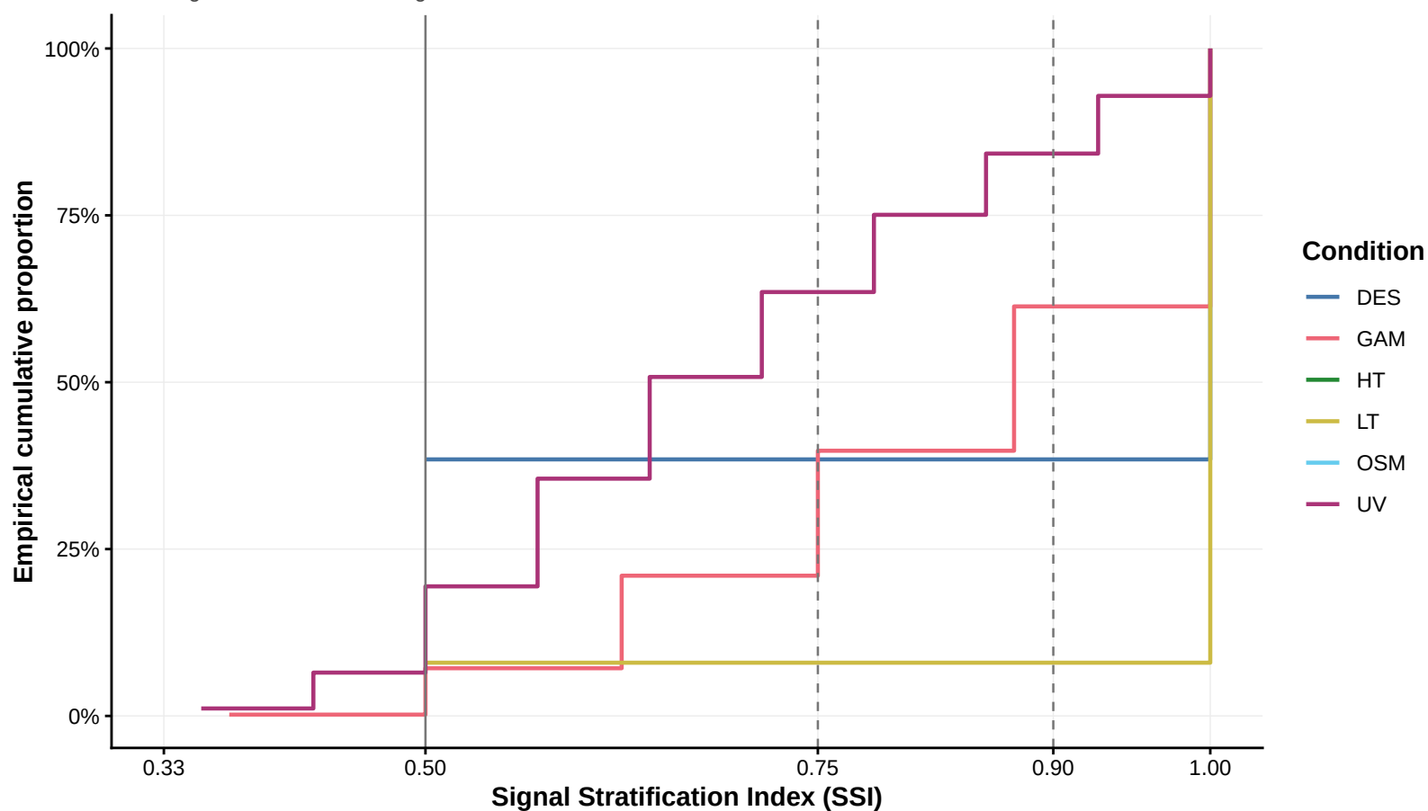
Figure 4. Empirical SSI distributions by condition
