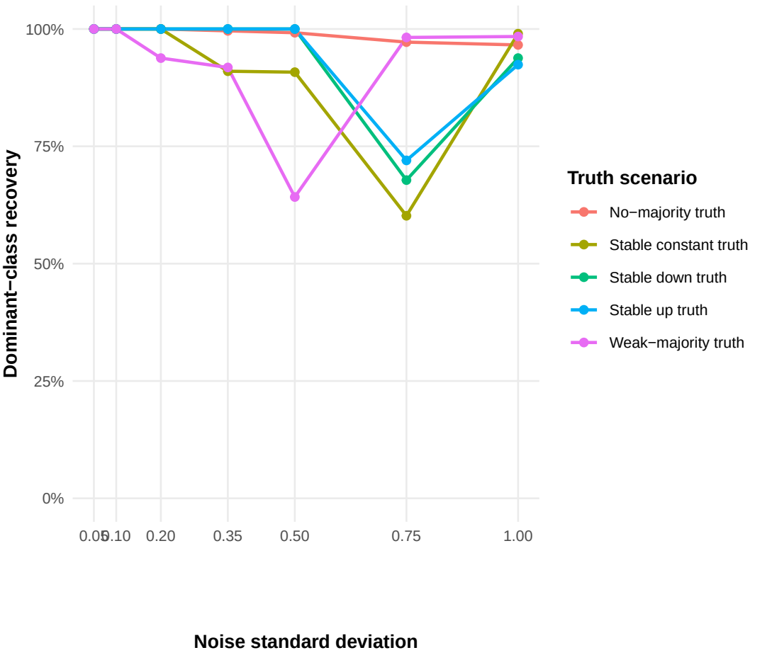
C. Recovery by truth scenario
