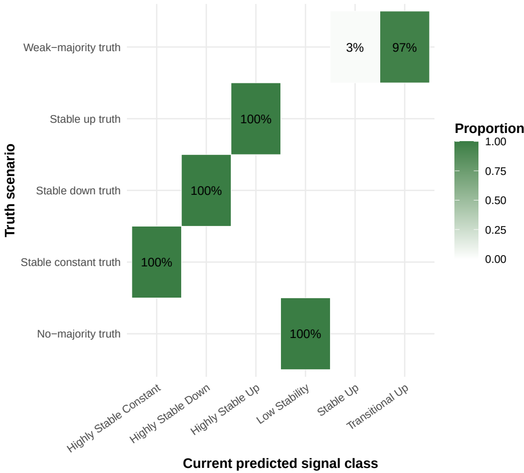
A. Baseline recovery
