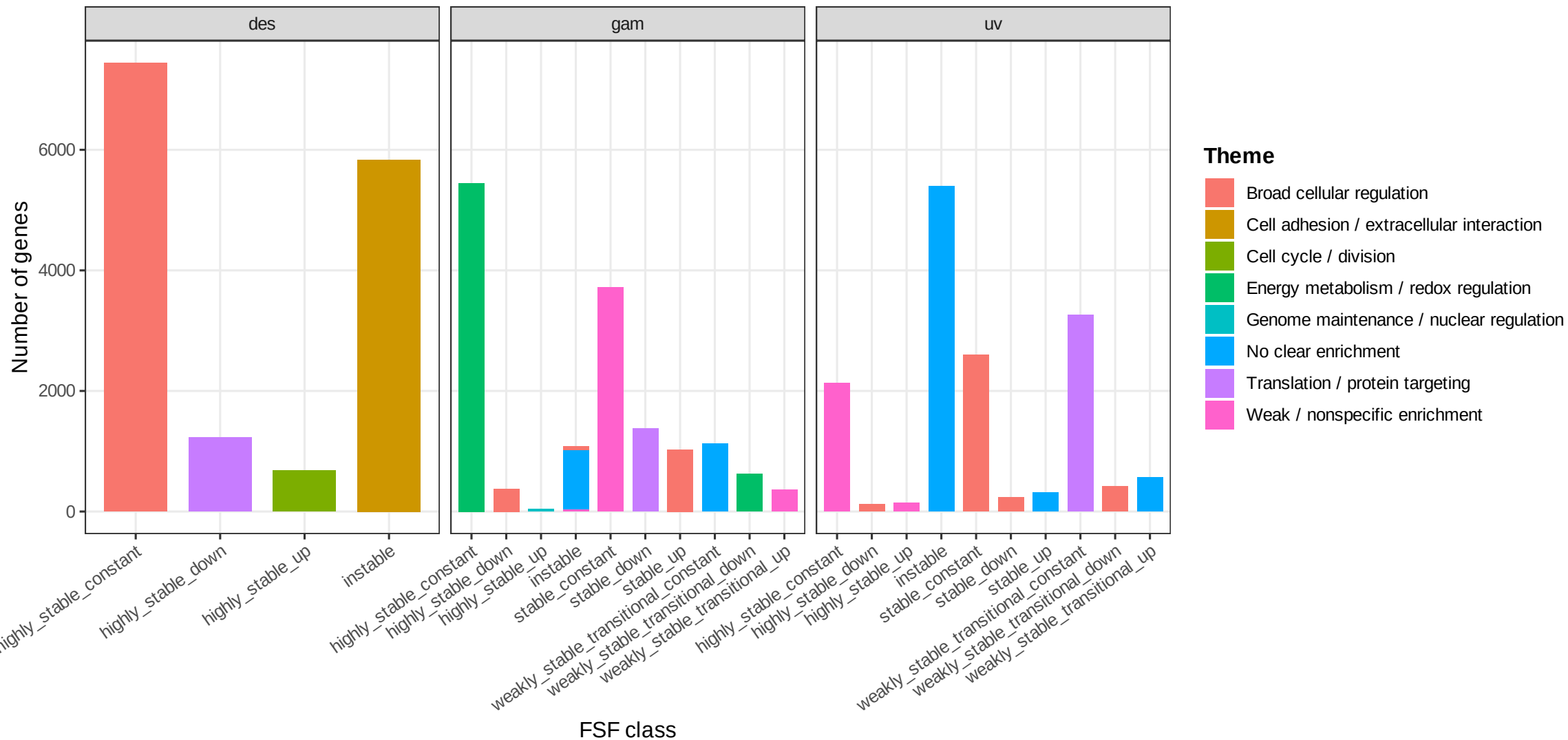
Figure 5C. Gene-weighted DES, UV and GAM biological profiles
