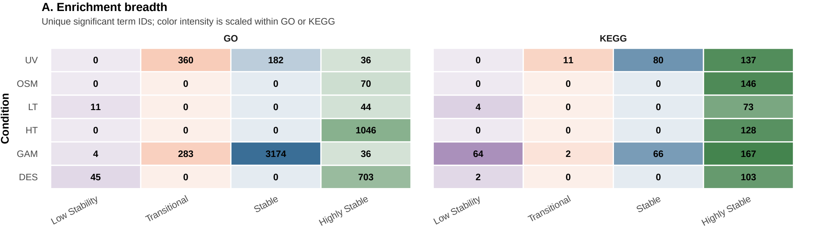
Figure 5. Functional enrichment evidence across FSF signal architectures
